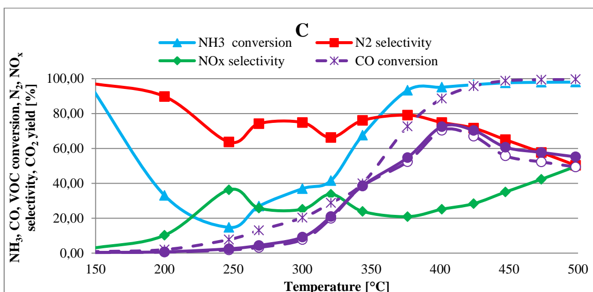
Fig. 4.8: NH_3 , CO, VOC conversion, N_2 and NO_x selectivity and CO_2 yield of sample C
