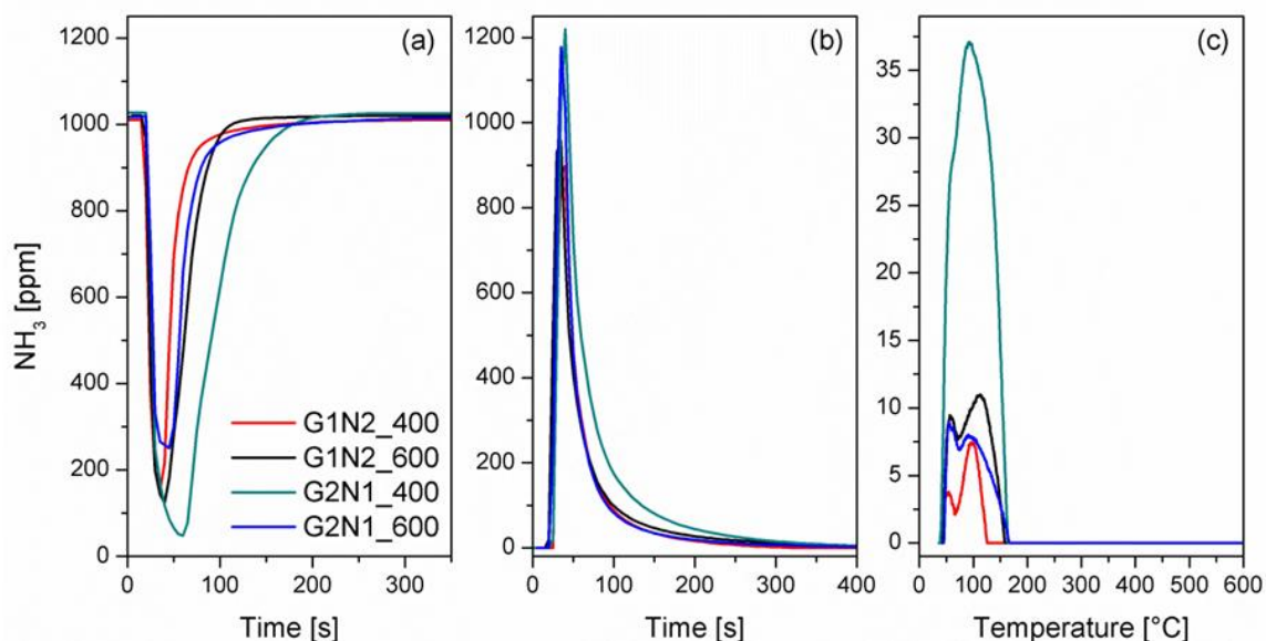
Fig. 3.4. \text{NH}_3 -TPD profiles: \text{NH}_3 adsorption curves at r.t. (a); \text{NH}_3 desorption curves at r.t. (b); \text{NH}_3 desorption curves at high temperature (c).
