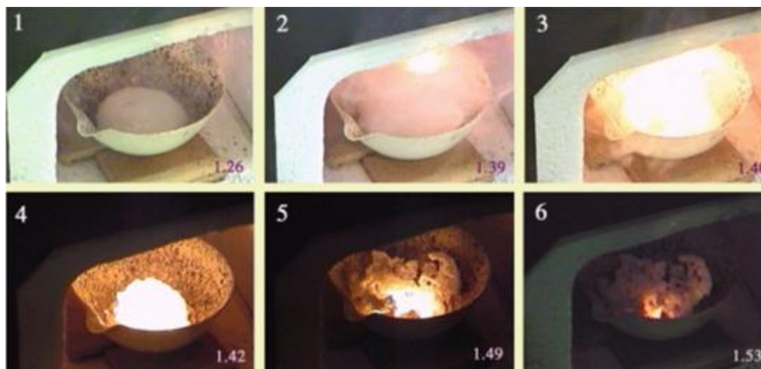
Fig. 3.1: SCS method.
