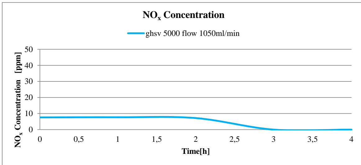
Fig. 4.37: NO x concentration for samples A under a total flow of 1050 ml/min and GHSV= 5000 h -1 .
