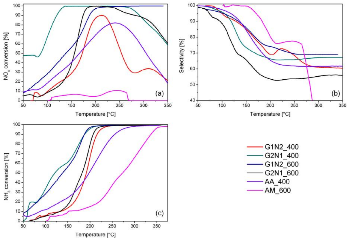
Fig. 3.6. Catalytic activity of the synthesized samples: (a) NO x conversion; (b) selectivity; (c) NH 3 conversion.
