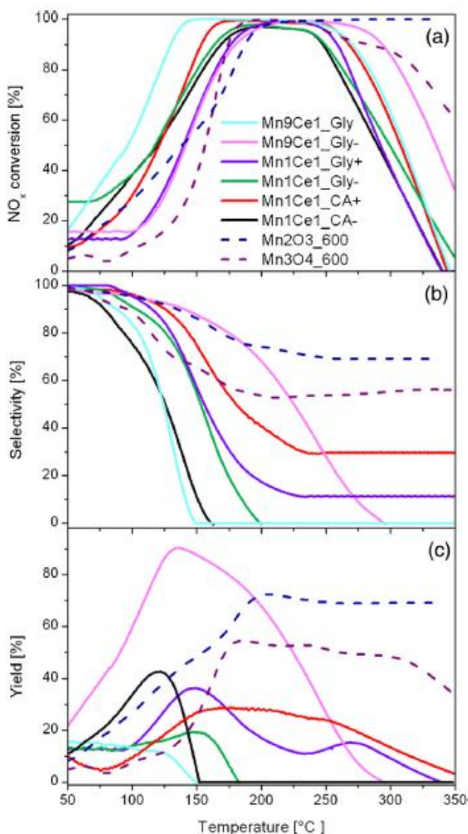
Fig. 3.14. Catalytic activity of the MnO_x-CeO_2 catalysts developed and of two MnO_x catalysts obtained by SCS [4]: (a) NO_x conversion; (b) selectivity; (c) yield.
