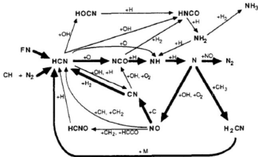
Fig. 1.5: Reaction path diagram illustrating the major steps in prompt \text{NO}_x formation and conversion of fuel nitrogen (FN) to NO.
