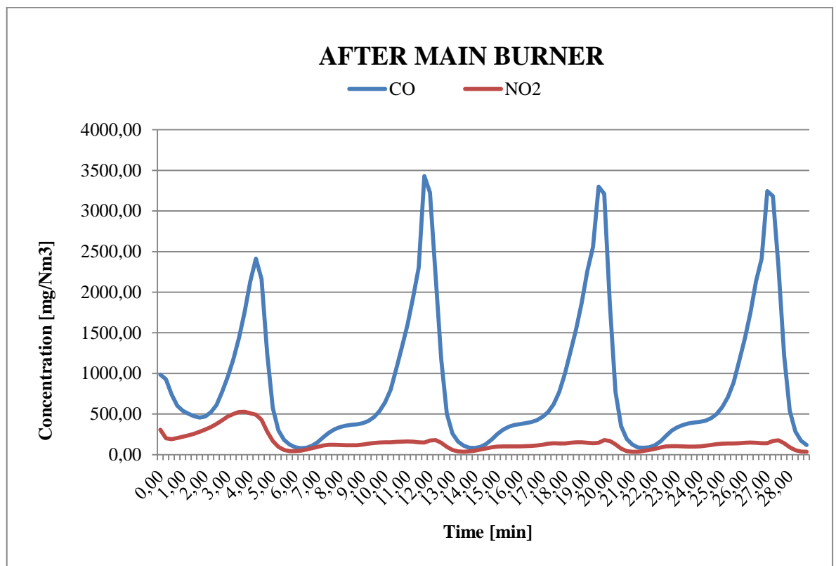
Fig.1.12: CO and NO 2 emissions after the main burner for a representative roasting cycle.
