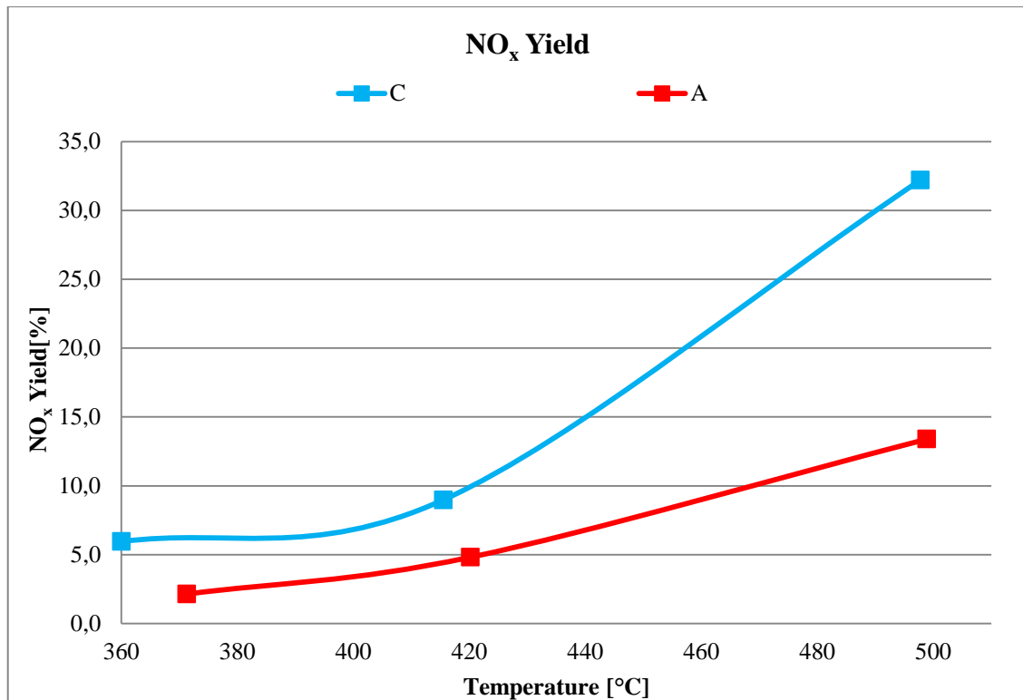
Fig. 4.31: NO x yield for samples A and C.
