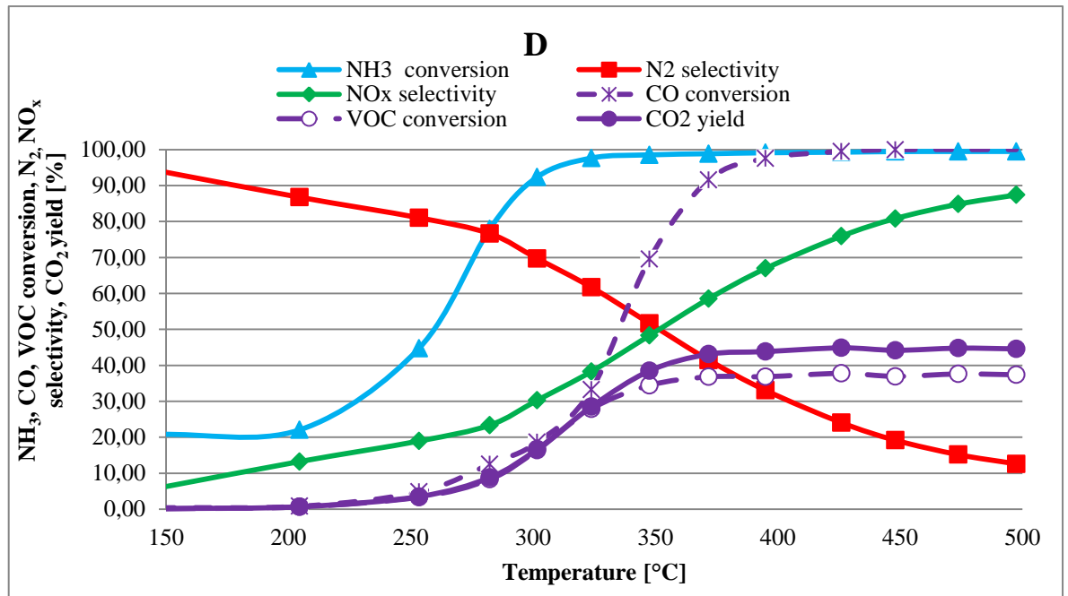
Fig. 4.9: NH 3 , CO, VOC conversion, N 2 and NO x selectivity and CO 2 yield of sample D
