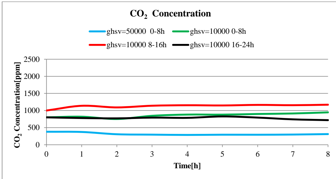
Fig. 4.33: CO 2 concentration for samples A at different GHSV.
