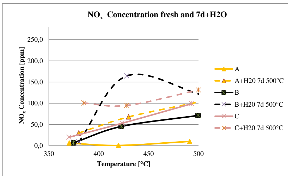
Fig. 4.28: \text{NO}_x concentrations for samples for samples fresh and treated 72d with water vapour.
