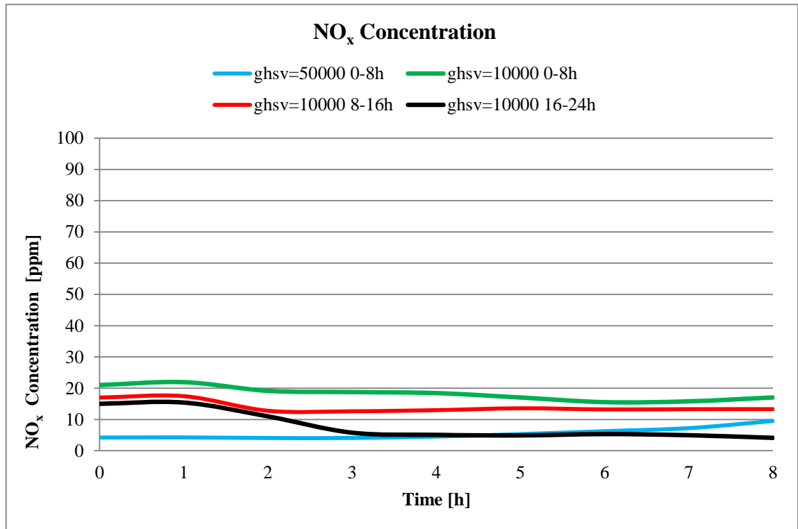
Fig. 4.35: \text{NO}_x concentration for samples A at different GHSV.
