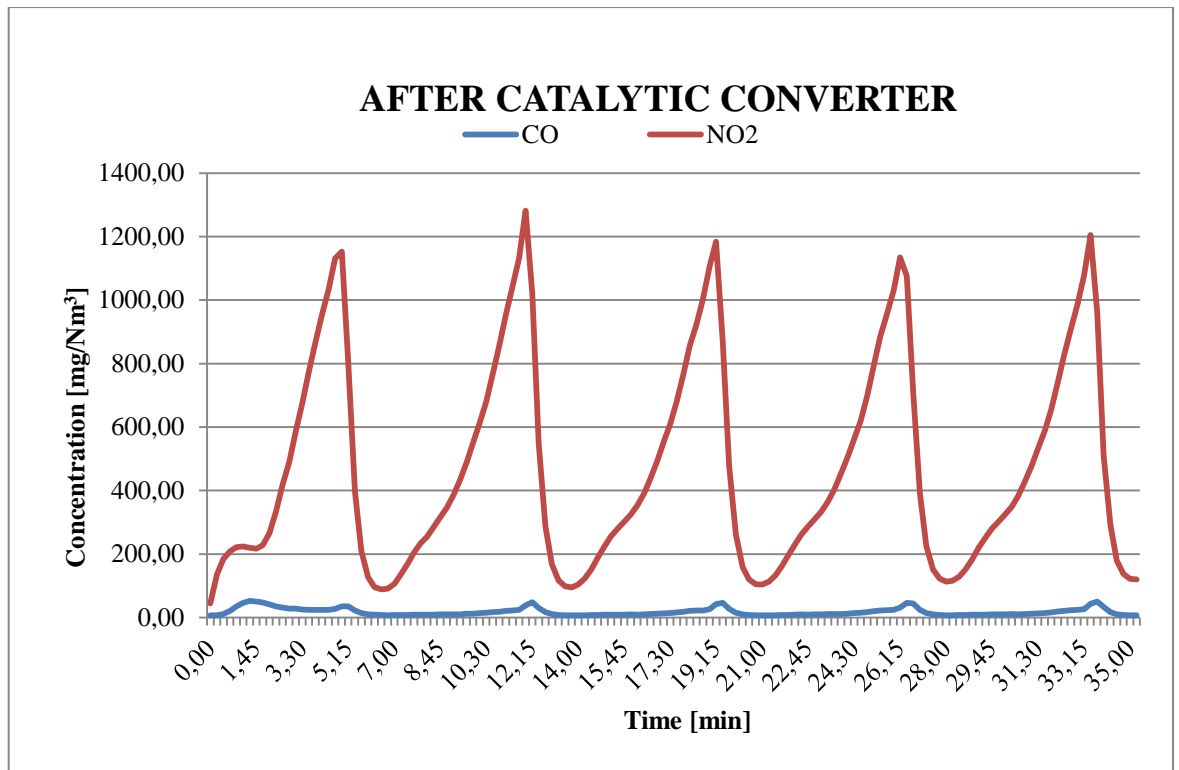
Fig.1.15: CO and NO 2 emissions after the catalytic converter for a representative roasting cycle.
