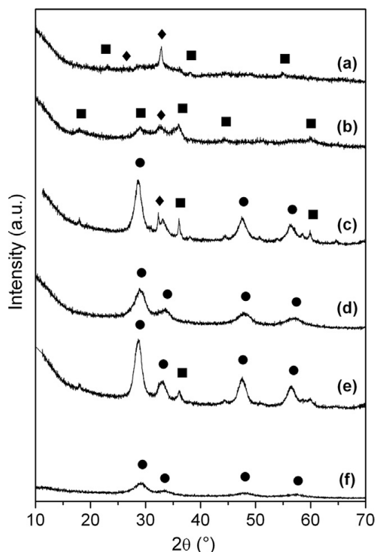
Fig. 3.10. XRD patterns of the MnO_x-CeO_2 catalysts developed: (a) Mn_9Ce_1 Gly, (b) Mn_9Ce_1 Gly - , (c) Mn_1Ce_1 Gly + , (d) Mn_1Ce_1 Gly - , (e) Mn_1Ce_1 CA + , (f) Mn_1Ce_1 CA - (■ Mn_3O_4 , ◆ Mn_2O_3 , ● CeO_2 ).
