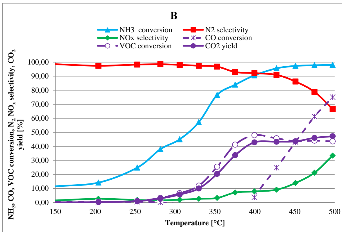
Fig. 4.7: NH_3 , CO, VOC conversion, N_2 and NO_x selectivity and CO_2 yield of sample B.
