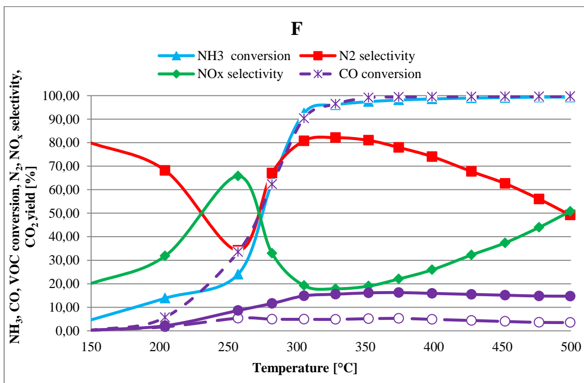
Fig. 4.11: NH 3 , CO, VOC conversion, N 2 and NO x selectivity and CO 2 yield of sample F
