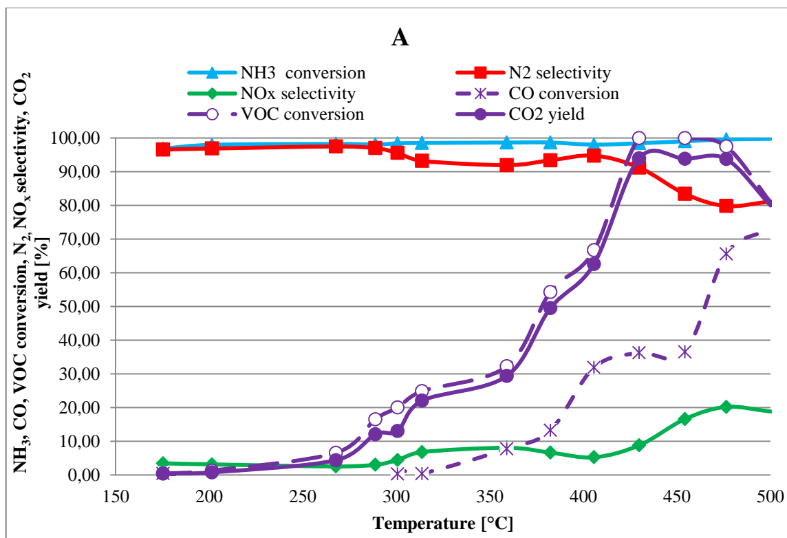
Fig. 4.6: \text{NH}_3 , CO, VOC conversion, \text{N}_2 , \text{NO}_x selectivity and \text{CO}_2 yield of sample A.
