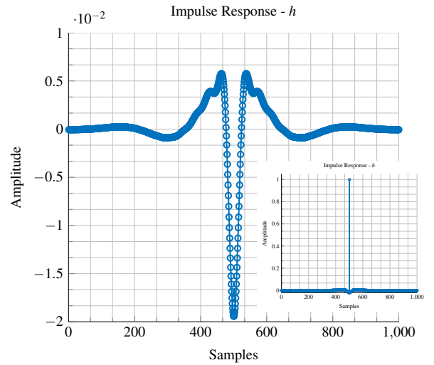
Figure 4. Impulse response of the minimum ISI FIR filter ( N=1001 , symmetric impulse response), omitting central unity tap. N_{\text{TWDM}} = 8 , P_{\text{TWDM}} = 9 dBm, depolarized signals. In inset, the full impulse response with the unity tap.
