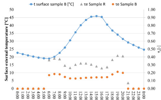
Fig. 5. Solar transmission coefficient of Samples B and R and surface temperature of Sample B.
