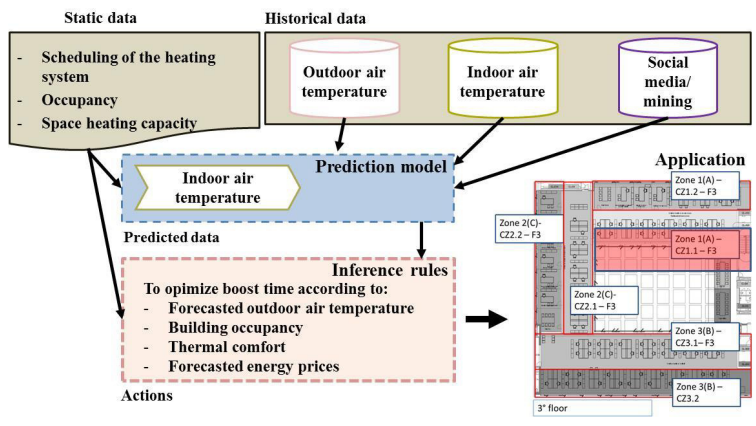
Fig. 4. Action modeling procedure scheme applied to the Town Hall of Sant Cugat, Barcelona, Spain.
