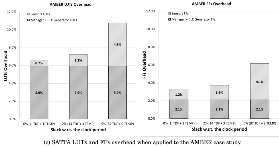
Fig. 13: FPGA hardware overhead when applying SATTA to the five case studies.
