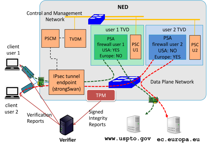
Fig. 1. A NED managing a multi-tenant scenario with different security policies enforced
