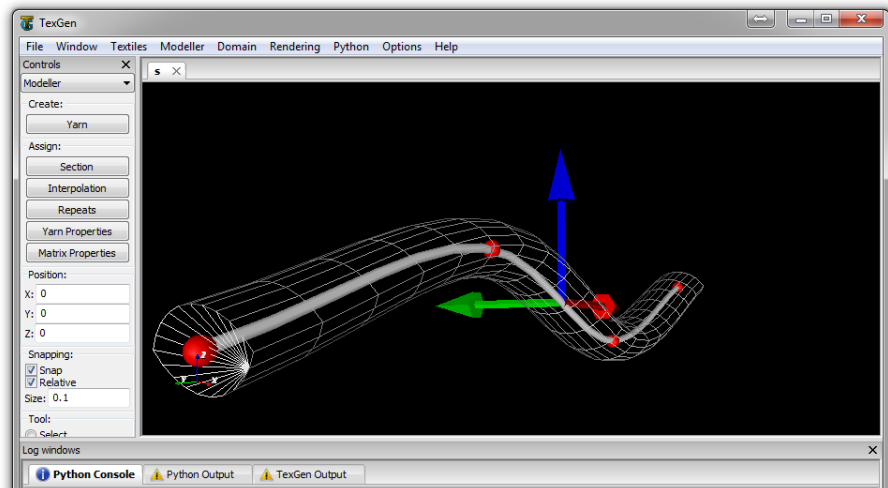
Figure 4.16 - TexGen yarn
