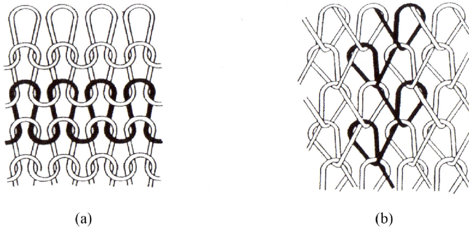
Figure 2.13 - Knitted fabrics: (a) weft knitted, (b) warp knitted
