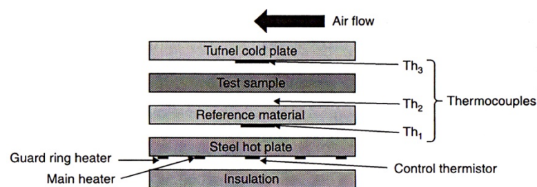
Figure 3.3 - Guarded hot-plate
