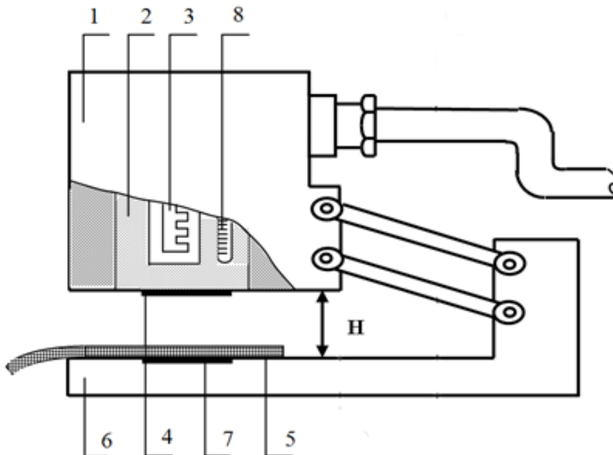
Figure 3.4 - ALAMBETA instrument
