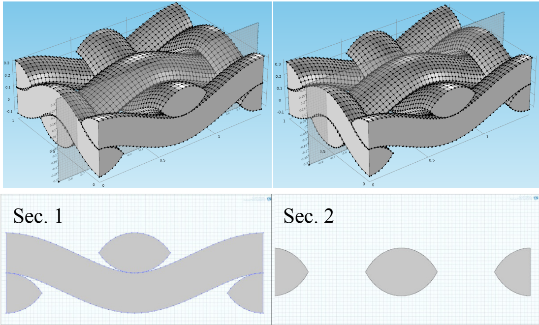
Figure 4.27 - Fabric sections used for simulations
