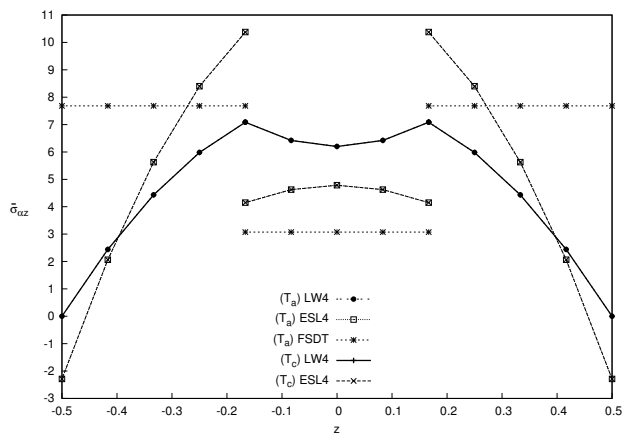
Figure 10: Transverse shear stress \sigma_{\alpha z} along the thickness, with thickness ratio ( a/h ) = 100. Composite plate.
