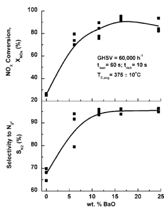
Fig. 12 Dependence of the time-averaged NO x conversion and selectivity to N 2 on BaO loading. The flow rate is 1 NI/min, the total cycle time is 70s (Reprinted from [84]).
