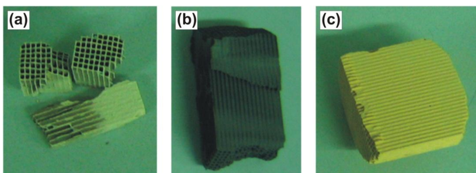
Figure 1. Commercial catalysts used for compatibility tests: diesel oxidation catalyst (a), soot oxidation catalyst (b), ammonia-SCR de- \text{NO}_x catalyst (c).
