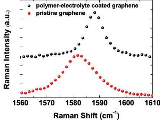
Figure 2.18. G-band Raman shift for pristine graphene and PES coated graphene.[26]
