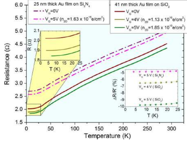
Figure 2.10. Temperature dependence of the resistance of two Au films for different values of the gate voltage. The corresponding values of n_{2D} , measured at room temperature, are indicated in the legend. Upper inset: zoom of the low temperature region. Lower inset: relative resistance variation \Delta R/R' at low temperatures, extracted from the curves in the main panel.[6]
