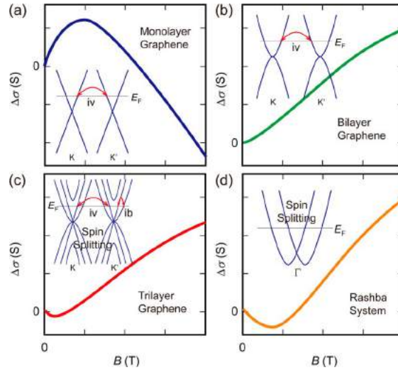
Figure 2.26. Schematic diagrams of \Delta\sigma as a function of magnetic field at low temperature limit. The curves in (a) and (b) are based on experiments done on monolayer and bilayer graphene; the curve in (c) is drawn from observations in three layer graphene EDL transistors, and the curve in (d) is from experiments on conventional Rashba system. Insets: band structures and elastic scatterings of carriers such as intervalley scattering (iv) and interband scattering (ib).[28]
