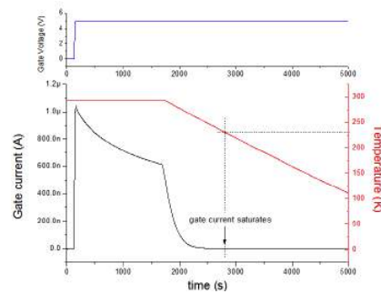
Figure 3.26. Top: Applied gate voltage; Below: Corresponding effect of the applied bias on the gate current plotted versus time at the decrease of temperature
