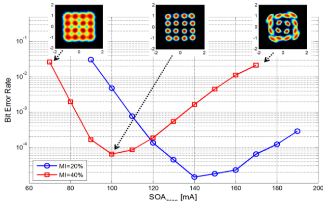
Fig. 7 Pre-FEC BER vs. SOA bias current, for a m_{index} of 0.2 and 0.4 and ODN loss of 25 dB.
