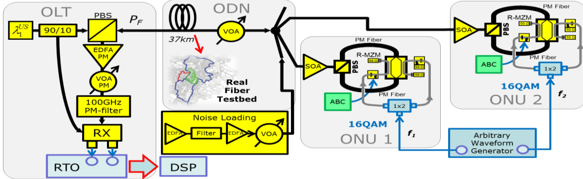
Fig. 5 Full experimental setup with installed fiber and two active ONUs. (PBS: Polarizing Beam Splitter, VOA: Variable Optical Amplifier, EDFA: Erbium Doped Fiber Amplifier, PM: Polarization Maintaining, RTO: Real Time Oscilloscope, DSP: Digital Signal Processing, SOA: Semiconductor Optical Amplifier, ABC: Automatic Bias Control, R-MZM: Reflective Mach Zehnder Modulator).
