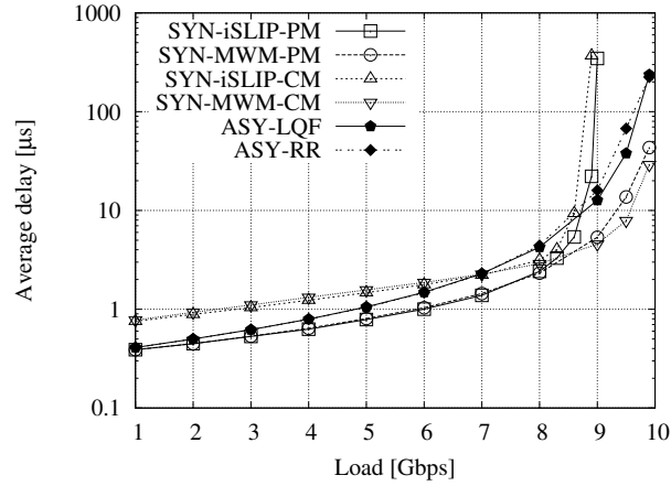
Figure 8: Average packet delay under bidiagonal traffic for the trimodal packet size distribution with N = 16 .
