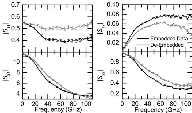
Fig. 1. Effect of the de-embedding on the calibrated S-parameters of a common-emitter InP DHBT, biased with 1.2 V collector-emitter voltage and with a base current of 400 \mu A ( 1\sigma uncertainty bars).
