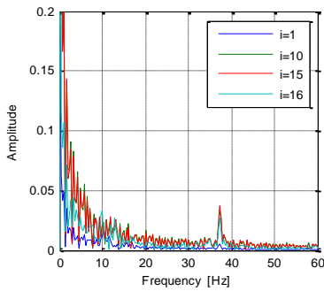
Fig. 9 Frequency spectrum at j=8 for J_l = 1.86 \text{ m/s} - J_g = 8.73 \text{ m/s}
