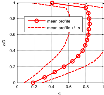
Fig. 8 Void fraction profile analysis for “non periodic with high noise” flow at J_l = 1.86 \text{ m/s} - J_g = 8.73 \text{ m/s}
