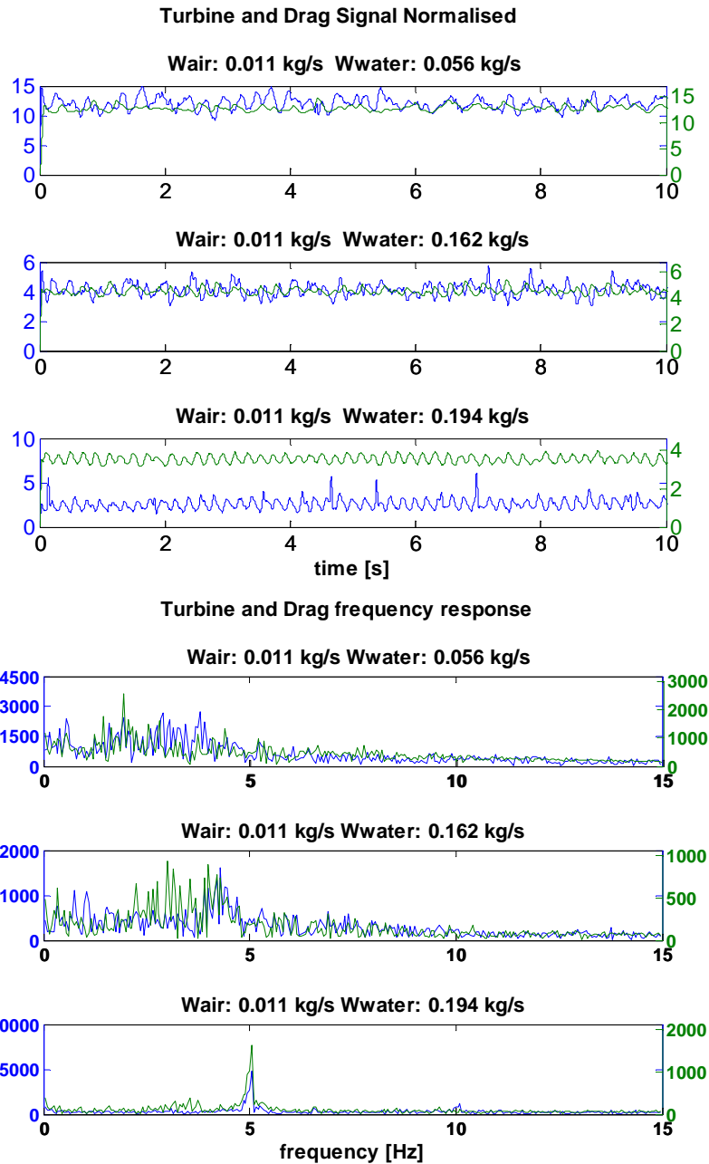
Fig.6.12: Time and Frequency Signal Analysis
