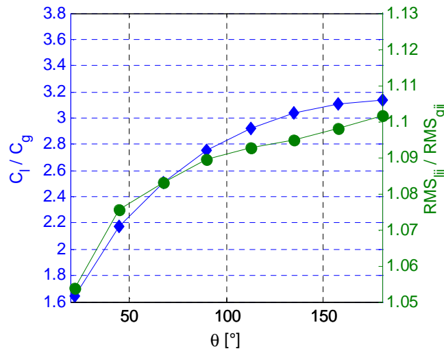
Fig.8.33: Comparison between experimental ( RMS_l/RMS_g ) and numerical ( C_l/C_g ) external electrodes response in single-phase conditions
