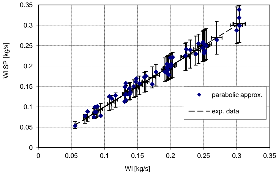
Fig.6.9: W_1 SP vs. Experimental W_1 . Error bar: y = \pm 15\% of Experimental W_1
