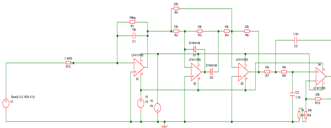
Fig.6.19: Electrical scheme. Measurement system
