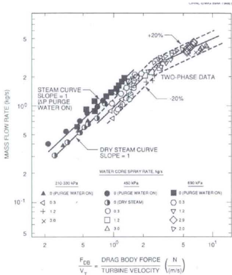
Fig.4.10: Comparison of mass flow rate from measured inputs with a mass flow model combining drag body and turbine meter measurement [4.26]
