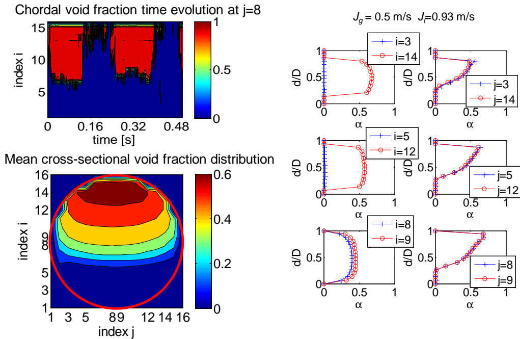
Fig.5.30: Plug flow example: J_f=0.93 \text{ m/s} and J_g=0.5 \text{ m/s}
