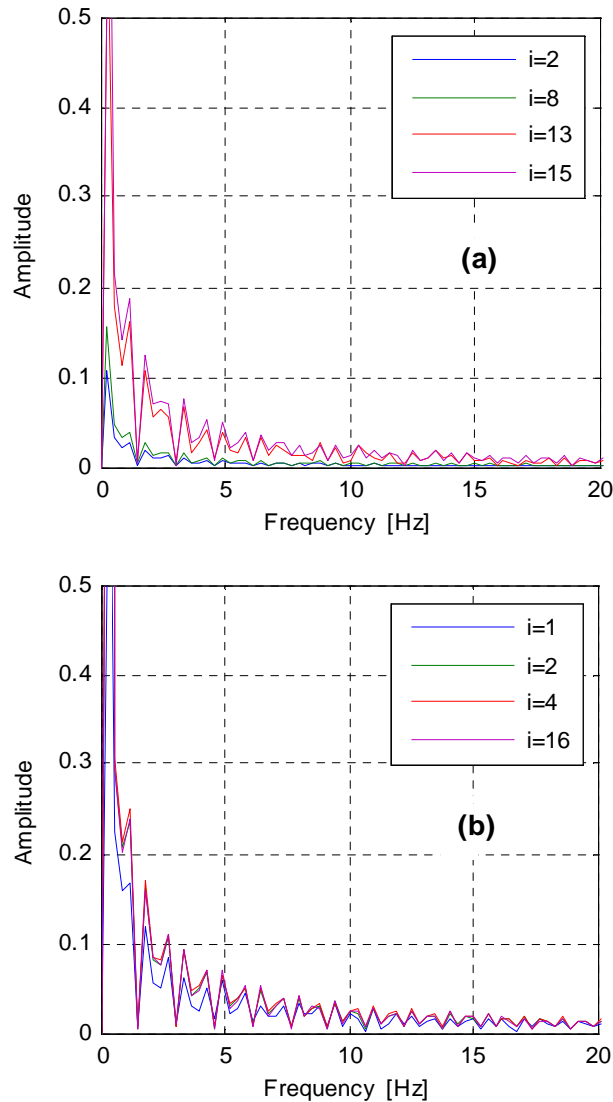
Fig.5.12: Frequency spectrum for non-intermittent flows. (a) J_g=0.23 m/s – J_t=1.86 m/s, (b) J_g=29.3 m/s – J_t=0.05 m/s
