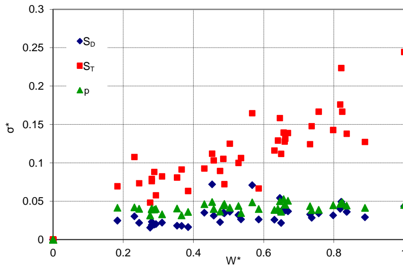
Fig.6.10: Standard deviation of electric signals
