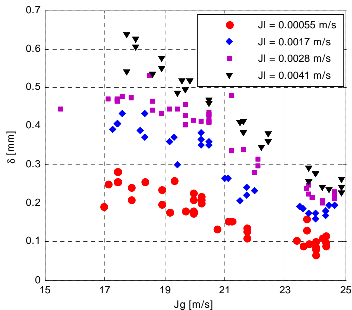
Fig.8.18: Corrected mean film thickness as a function of the experimental water and air superficial velocities
