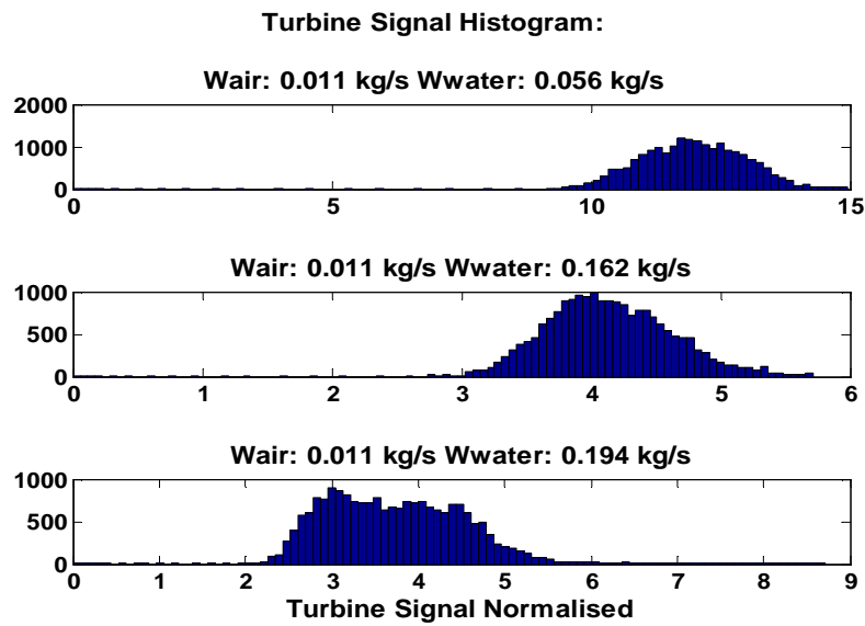
Fig.6.11: Signal Histograms
