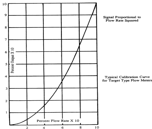
Fig.4.5: Typical Calibration Curve for Target flow Meters
