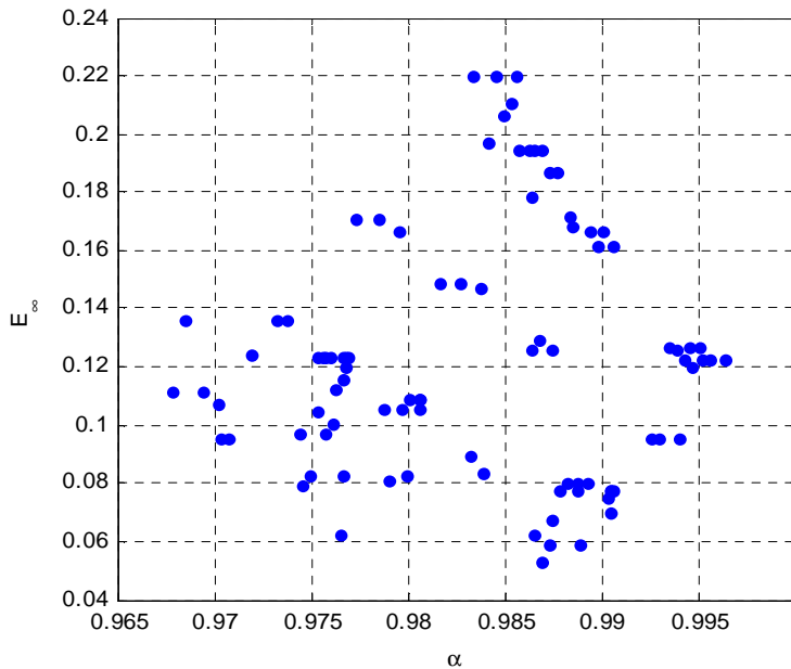
Fig.8.14: Equilibrium entrainment (eq. 8.5) as a function of the experimental volumetric void fraction \alpha
