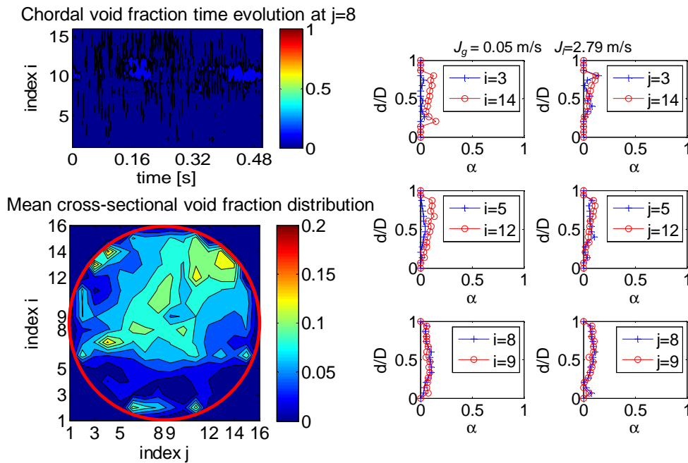
Fig.5.32: Bubbly flow example 2: J_1=2.79 m/s and J_g=0.05 m/s
