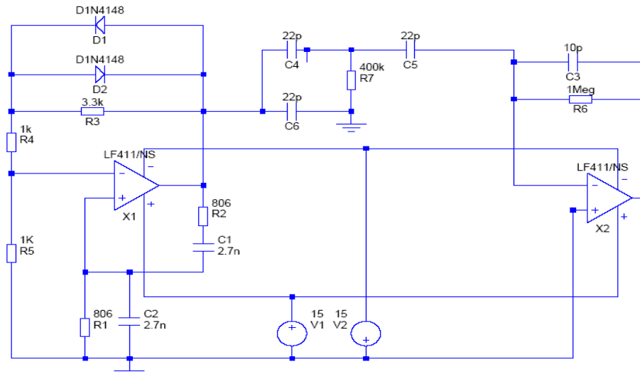
Fig.6.18: Electrical scheme. Oscillator
