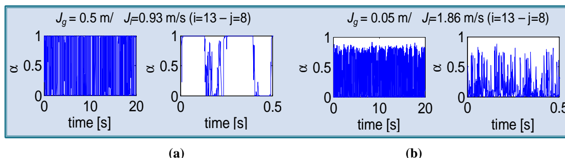
Fig.5.29: Void fraction time evolution at the point (13, 8) of the WMS grid at J_l = 0.93 and J_g = 0.5 m/s (a) and J_l = 1.86 and J_g = 0.05 m/s (b)
