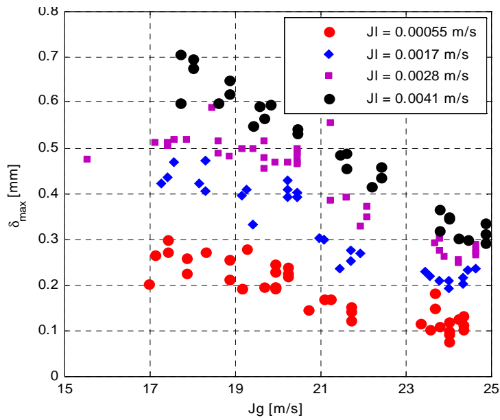
Fig.8.13: Maximum film thickness (eq. 8.8) as a function of the experimental water and air superficial velocity
