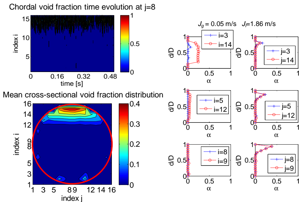
Fig.5.31: Bubbly flow example 1: J_f=1.86 \text{ m/s} and J_g=0.05 \text{ m/s}
