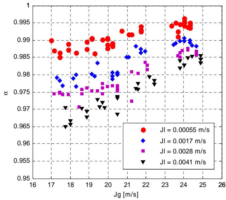
Fig.8.4: Experimental volumetric void fraction as a function of water and air superficial velocities
