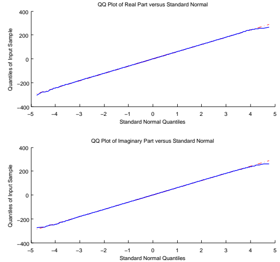
(b) Quantile-quantile plot.
