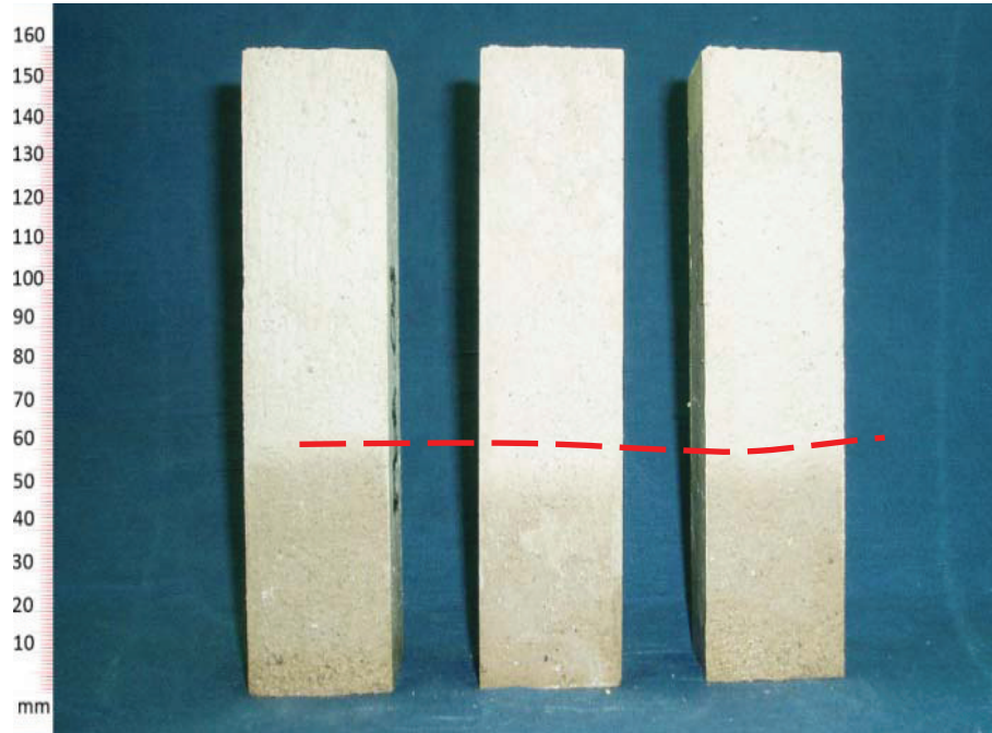
Fig. 12 Lift height of capillarity in specimens mortor A.
