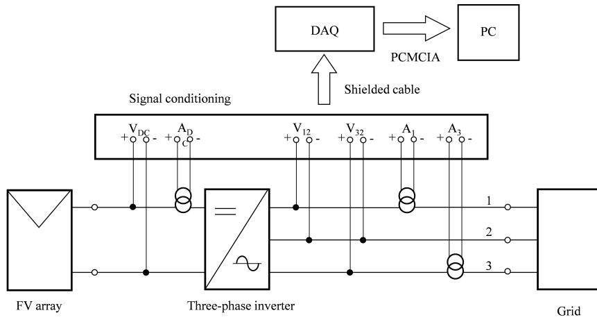
Figure 5.9: Measurement scheme for 230 kVA inverter.
