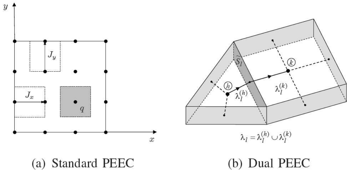
Figure 15 (a) Standard 2D discretization of current density (dashed cells) and charge density (gray cell), (b) dual discretization: the couple primal edge (straight line)/dual face (dark gray) correspond to a two terminal circuit component.
