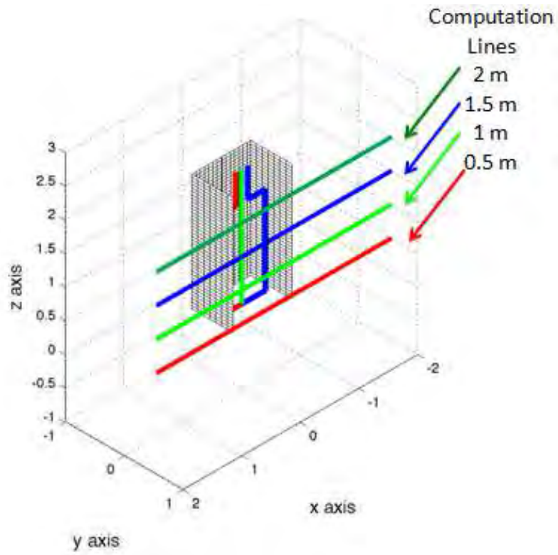
Figure 44 Layout of the shielding system u-shaped rear closed with computation lines and source layout
