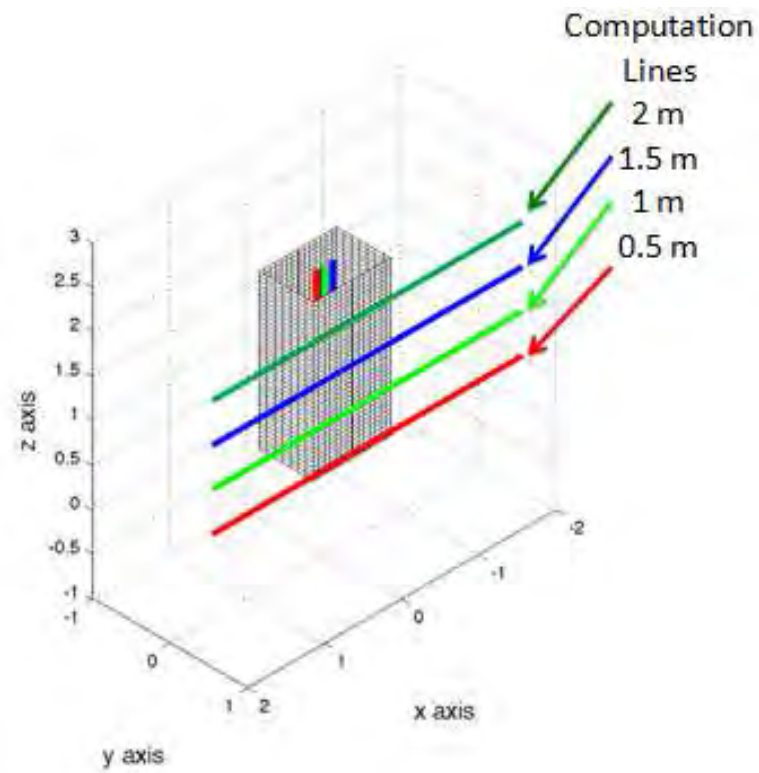
Figure 45 Layout of the shielding system closed on all 4 sides with computation lines and source layout
