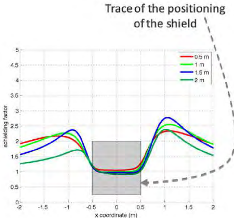
Figure 49 Shielding factor provided by u-shaped shield rear closed
