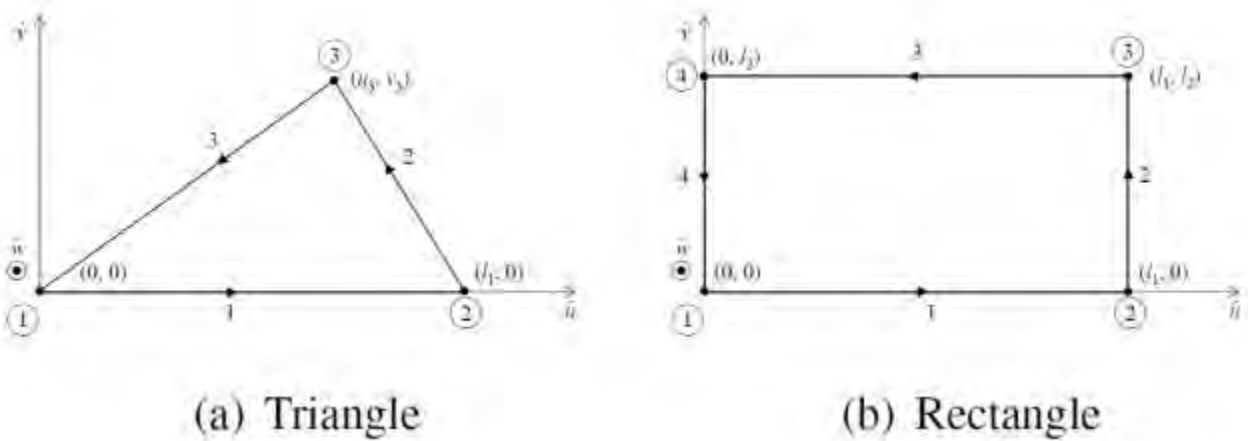
Figure 16 Plane triangle and rectangle in local frame (u; v; w) .
