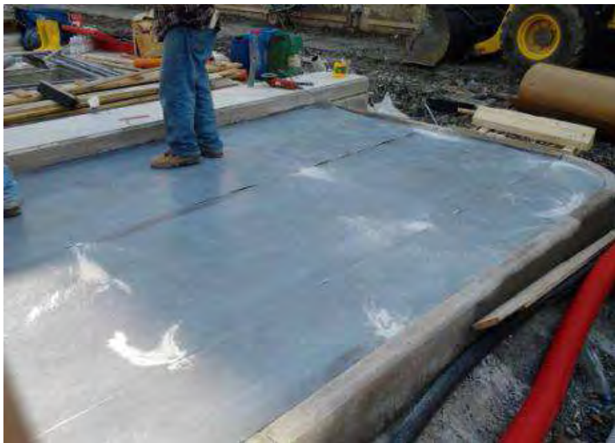
Figure 34 Image of the shielding system completed
