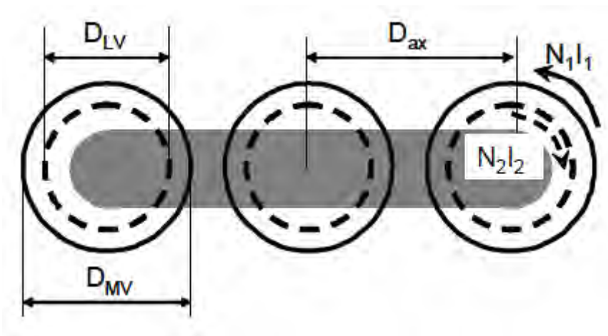
Figure 6 Characteristic geometric parameters for the evaluation of external magnetic fields
