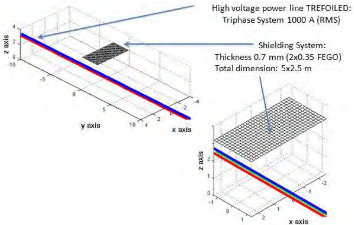
Figure 29 Layout used for the simulations
