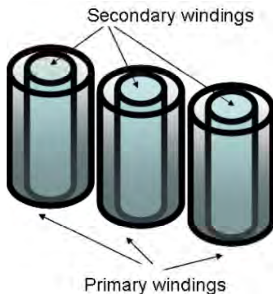
Figure 2 Primary and secondary windings
