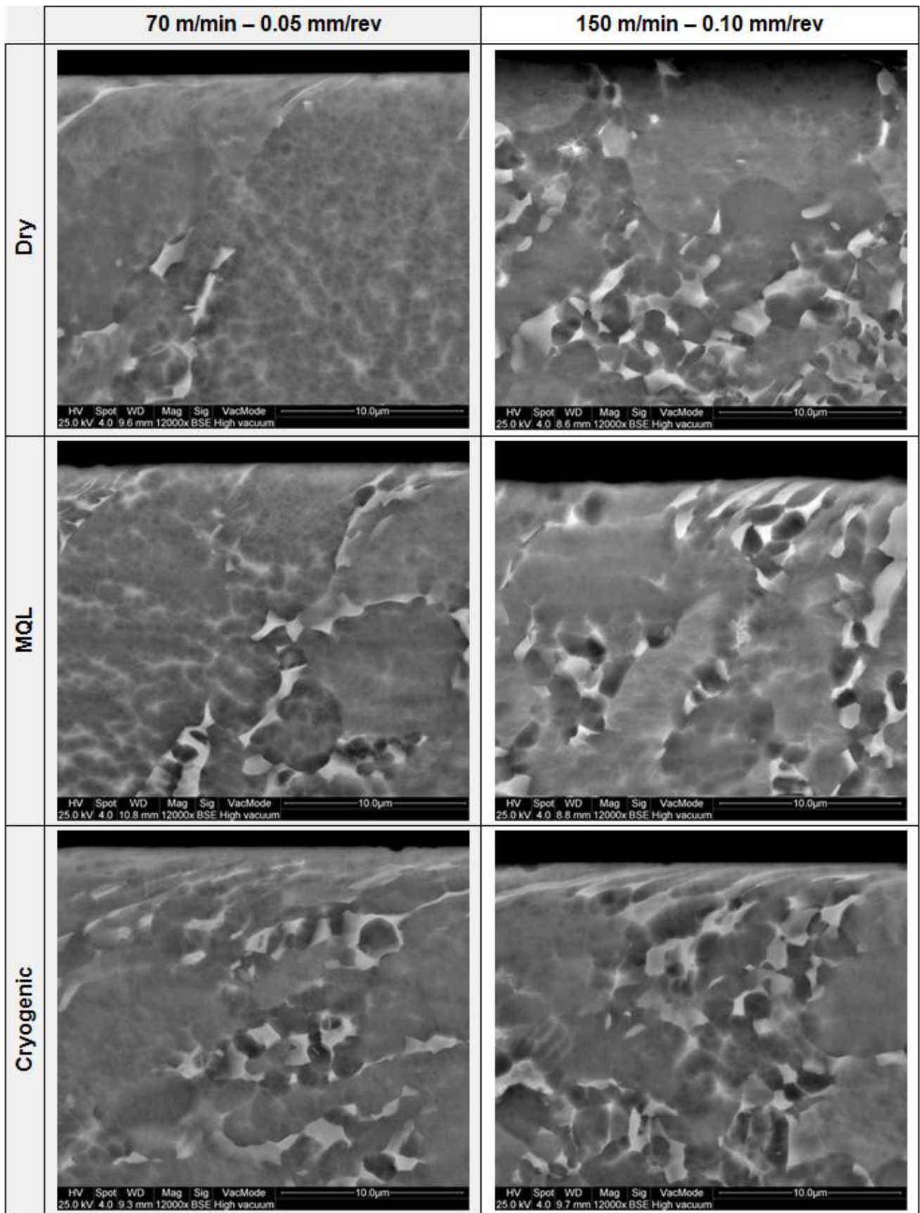
Figure 7. SEM images of the machined samples under dry, MQL, and cryogenic conditions at different cutting speeds and feed rates ( \alpha – dark grains; \beta – light grains).
