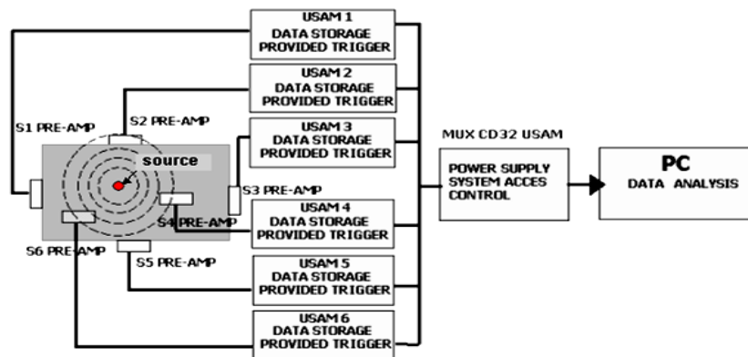
Figure 6: AE acquisition system.
