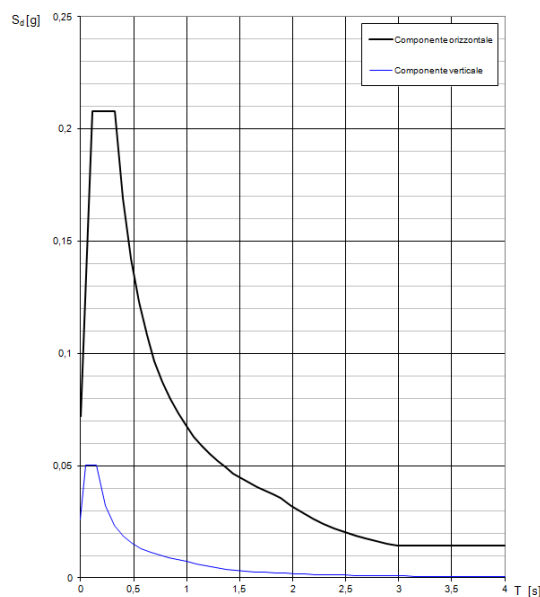
Figure 11: Elastic response spectrum of acceleration S_d (g).
