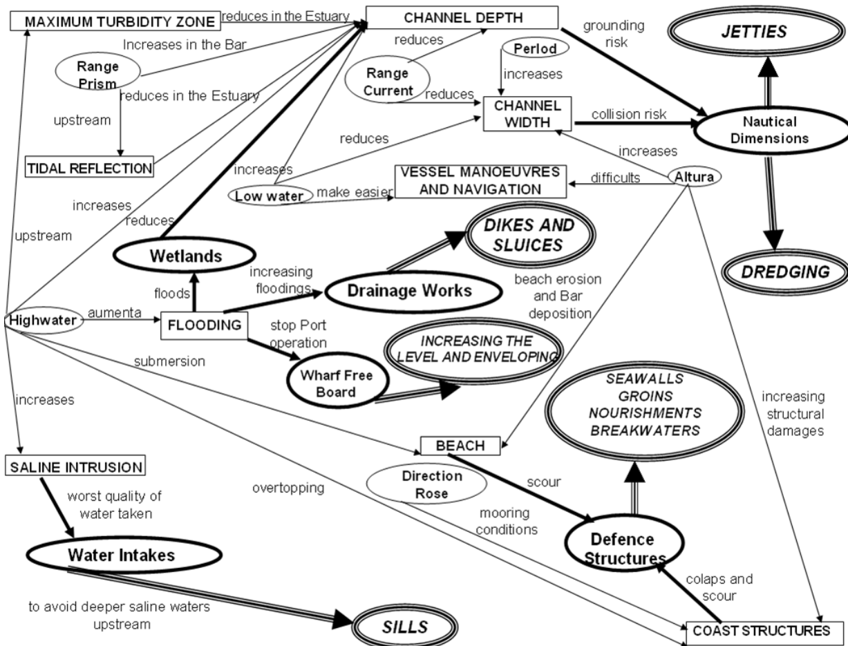
Figure 7 Frame of hydrodynamics for impacts on coastal and estuarines port areas and mitigatory measures and structures
