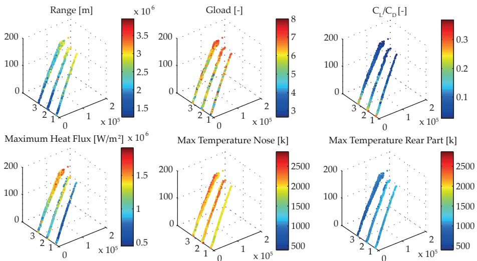
Figure 5.24 Performance trends on the Robust Pareto front.
