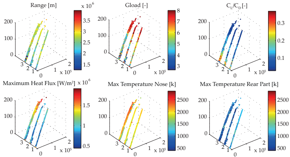
Figure 5.23 Performance trends on the Pareto front.
