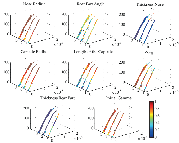
Figure 5.25 Variables trends on the Pareto front.
