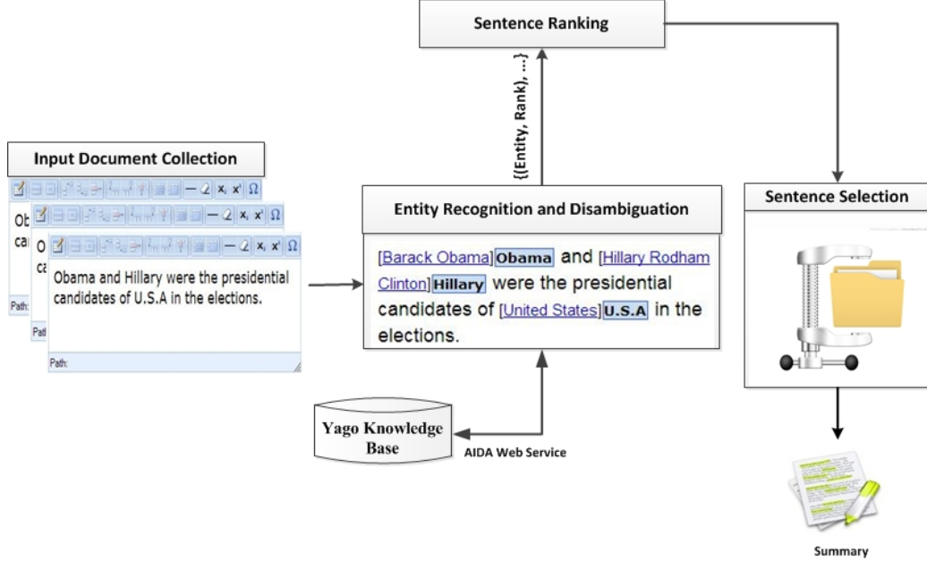
Figure 1: The Yago-based Summarizer.
