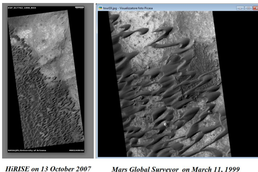
Fig.1 – The images of the Nili Patera dune field that we use here for the study of the moving dunes on Mars.
