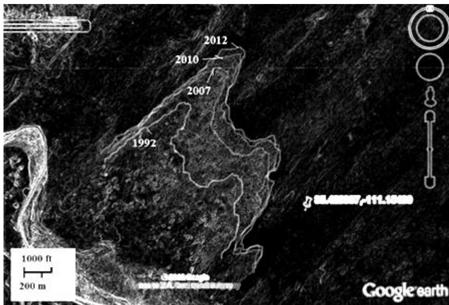
Figure 12 – Superposition of the images from Google Earth recorded at four different times (9/22/1992, 6/21/2007, 9/10/2010, 6/4/2012), after processing with GIMP. The fronts of the field of dunes are labeled with years.
