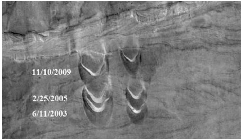
Figure 9 - Two moving dunes
