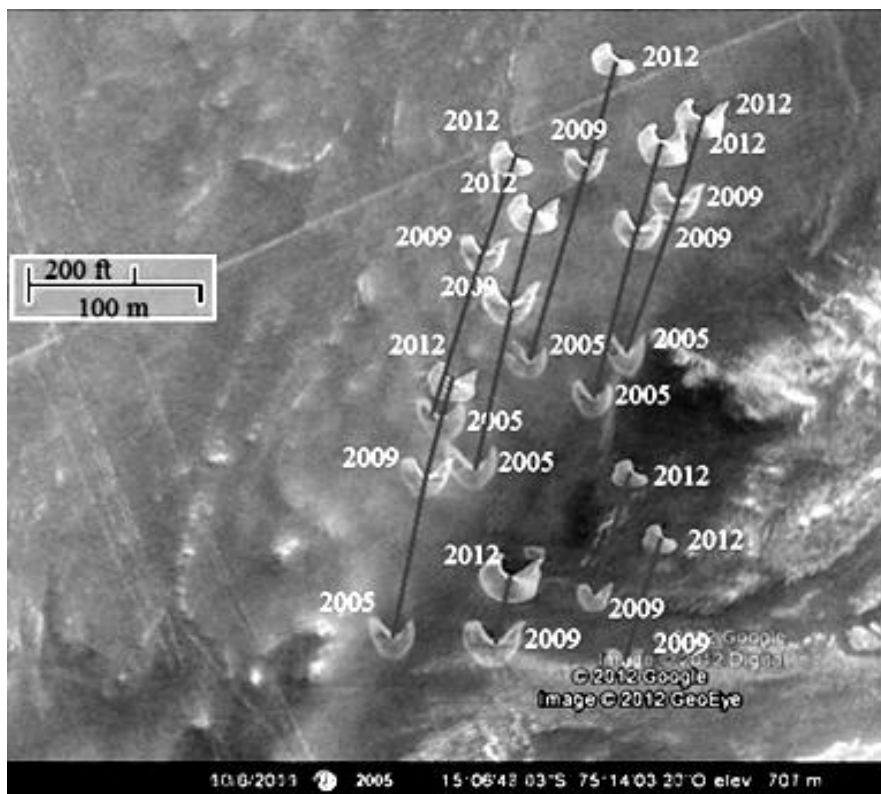
Figure 6 – Motion of barchans. The path of the dunes is given by the black lines, connecting the different positions labeled with years. Note that the small dunes move faster.
