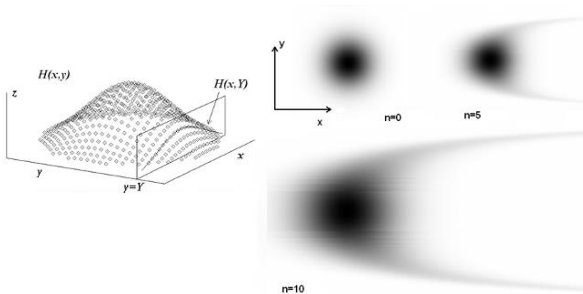
Figure 2 - At the beginning, we have a heap of sand with a Gaussian profile H(x,y) on the horizontal surface x,y . The profile of the dune is represented by means of grey tones corresponding to H . The white tones correspond to H=0 , whereas the black tones to H=1 . The radius of the heap is R=250 (arbitrary units). The height is H_0=1 (arbitrary units). The wind is blowing in the x -direction. For each vertical plane with fixed y=Y , the profile of the heap changes. The dimensionless height of the corresponding profile is h(Y)=\max(H(x,Y)/H_0) . The dimensionless velocity of the layer is v(Y)=1/h(Y) , inversely proportional to the height of the profile H(x,Y) of the dune corresponding to y=Y . We can see then the evolution of the dune as a function of time. Assuming the time step as \Delta t = R/50 (arbitrary units), after n steps, each layer H(x,Y) moves of different distances with respect to the others.
