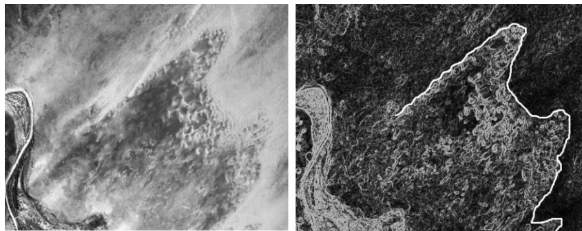
Figure 11 – On the left the field of dunes in the Google Earth images of 2007. On the right, same image after edge detection. The front is marked with a white line.
