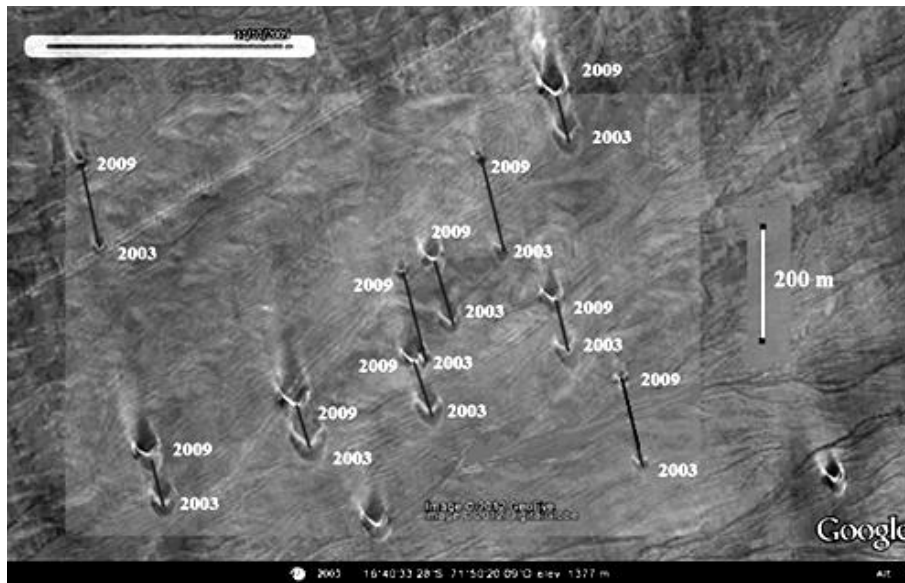
Figure 7 – Combining the images of 2003 and 2009 we can evaluate the speed of each dune.
