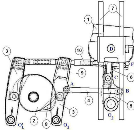
Figure 1: Sketch of the mechanism that moves the press bed.
