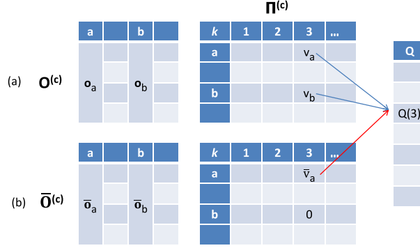
Fig. 2: Merging two rows of a matrix \mathbf{\Pi}^{(c)} having two non-zero values in the same column: (a) initial configuration, (b) updates of matrix \mathbf{\Pi}^{(c)} and \mathbf{O}^{(c)} according to steps 2 and 3 of Algorithm 2.
