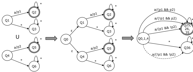
Figure 4. Example of a pFSA with complex predicates: the union case.
