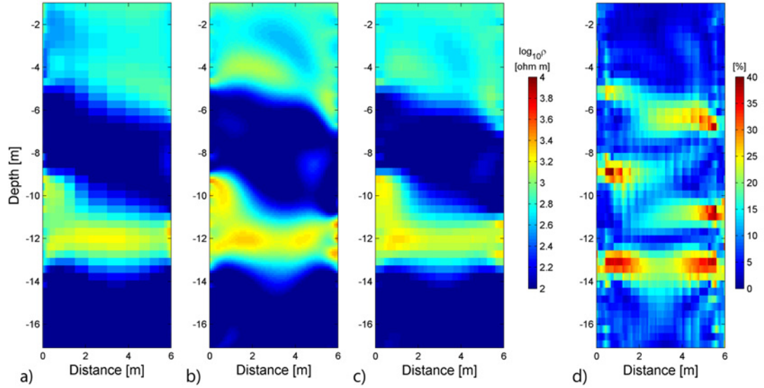
Fig. 2.5: synthetic model n.2, data with 5% noise; resistivity image from inversion of a) coarse irregular grid b) fine regular grid and c) image of averaged resistivity from SGERT; d) relative standard deviation image from the SGERT inversion.
