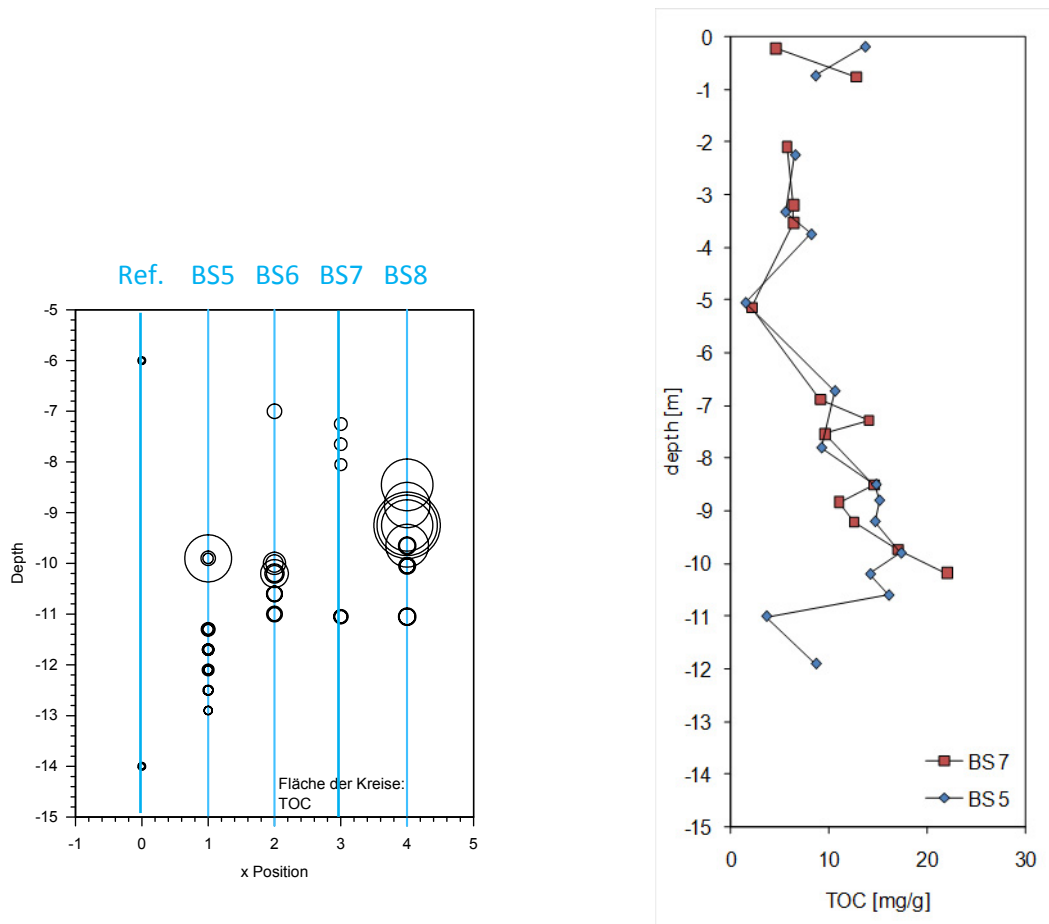
Figure 5.8: TOC a) in the groundwater in the ports of BS5 to BS8 on three sampling campaigns and b) in the solid phase of liners from BS 5 and BS 7. Area of the circles corresponds to TOC concentration in mg/l in the pore water. Background values were measured in the uncontaminated location, about 200m distance far (Courtesy M. Wehrer, Jena).
