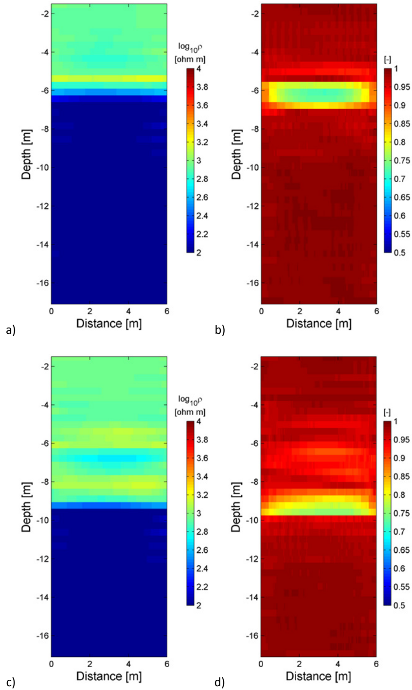
Fig. 4.5: Synthetic time-lapse model n. 2 (noise-free data), results from the SGERT inversion: image of average resistivity for the background (a) and the subsequent (c) case, precision P_0 (b) and P_t (d).
