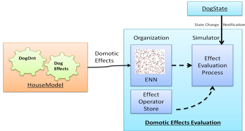
Figure 8. Logical architecture of Domotic Effects Evaluation bundle
