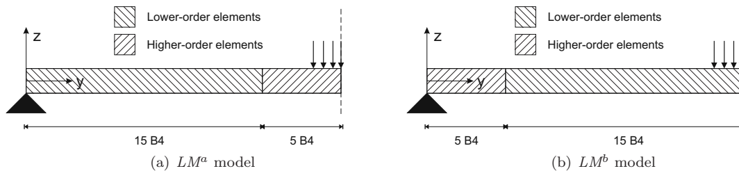
Figure 10: Variable kinematic models with refined elements near (a) the loading application zone or (b) the constraint
