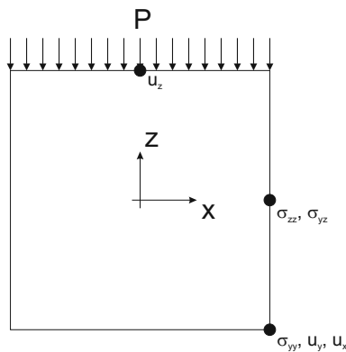
Figure 9: Square cross-section geometry, load and verification points
