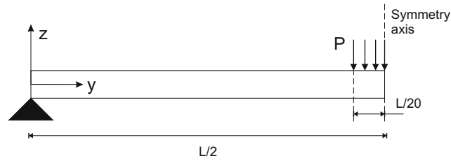
Figure 8: Simply supported beam under a localised uniform pressure P
