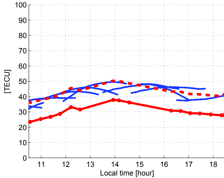
Figure 11.23: vTEC measurements, comparison between Ashtech receiver (blue), Arcibo ISR (red, solid line) and Arcibo ISR shifted by +12.5 TECU (red, dash line) for comparison purposes. March 27 th 2011.
