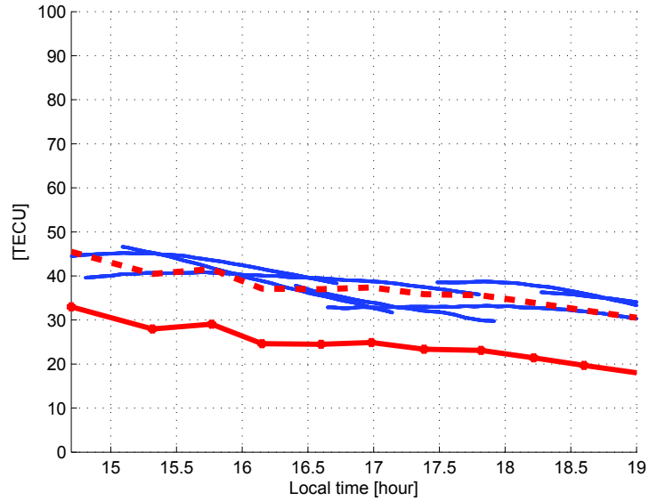
Figure 11.22: vTEC measurements, comparison between Ashtech receiver (blue), Arcibo ISR (red, solid line) and Arcibo ISR shifted by +12.5 TECU (red, dash line) for comparison purposes. March 25 th 2011.
