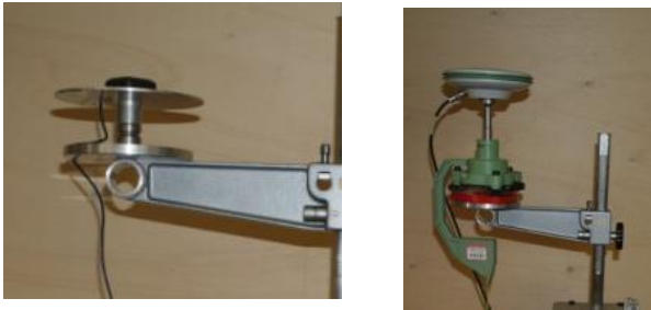
Figure 13. Antenna support: patch (left) and geodetic (right)
