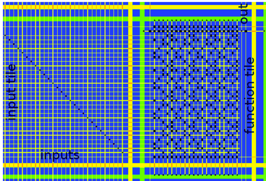
Figure 6: 28 input logic function layout.
