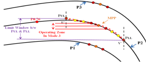
Fig. 11. Operation zone of different power curves
