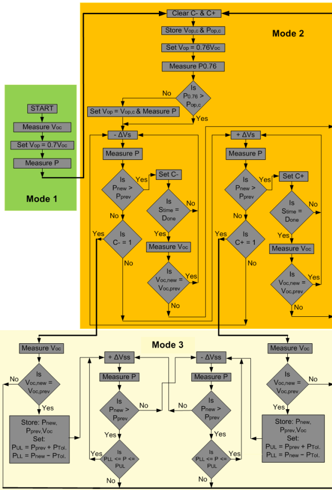
Fig. 5. Proposed Algorithm
