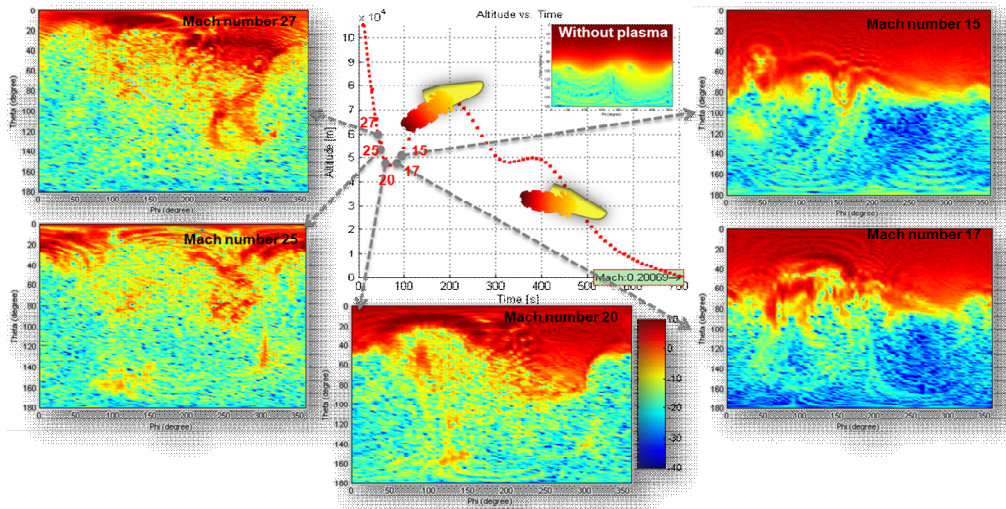
Fig. 4. Evolution of the IXV antenna gain in the critical region
