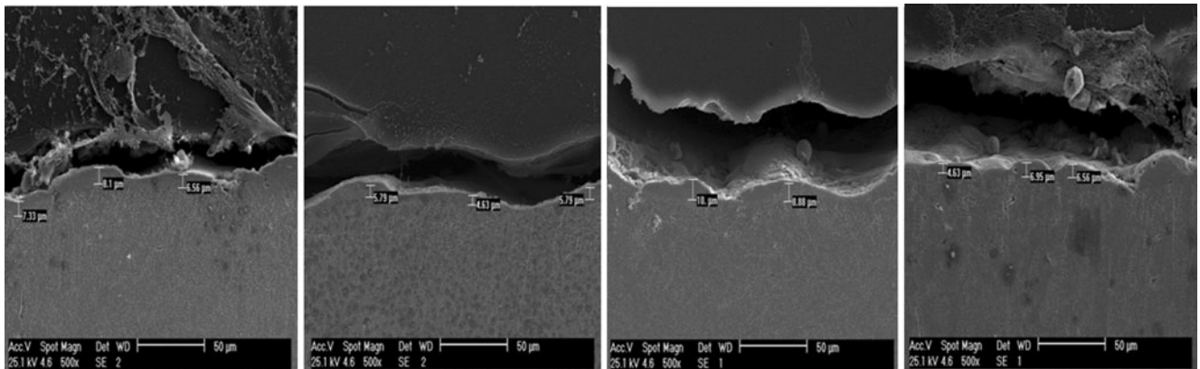
Fig. 5 Sequence of recast layer measurements performed by SEM in: run 1, without and with CNTs, run 2 without and with CNTs
