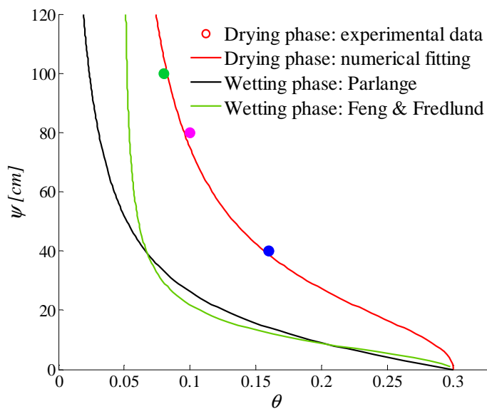
Fig. 28 – Test 2, soil water retention curve, main drying and main wetting branches
