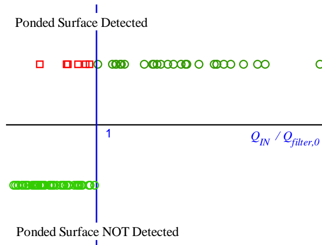
Fig. 70 – Measured and predicted occurrence of the storage phase for Cell 1 of the biofiltration facility installed at Monash University.
