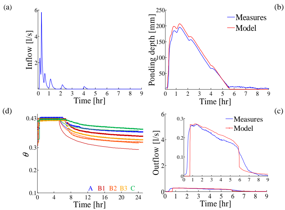
Fig. 42 – Event A: (a) Inflow hydrograph, measures; (b) Pondering depth time serie, measures and model; (c) Outflow hydrograph, measures and model; (d) Soil moisture time series, measures and model
