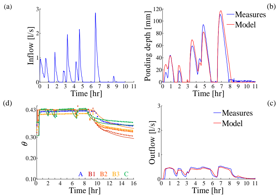
Fig. 74 – Event S*: (a) Inflow hydrograph, measures; (b) Pondering depth time serie, measures and model; (c) Outflow hydrograph, measures and model; (d) Soil moisture time series, measures and model
