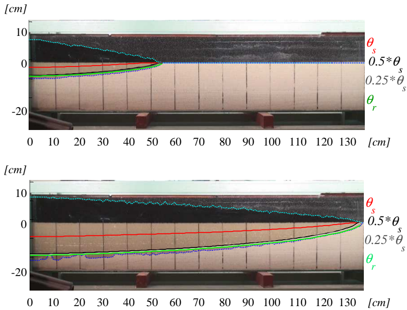
Fig. 31 – Detected and modeled wet/dry interfaces in the porous mat and in the sand
