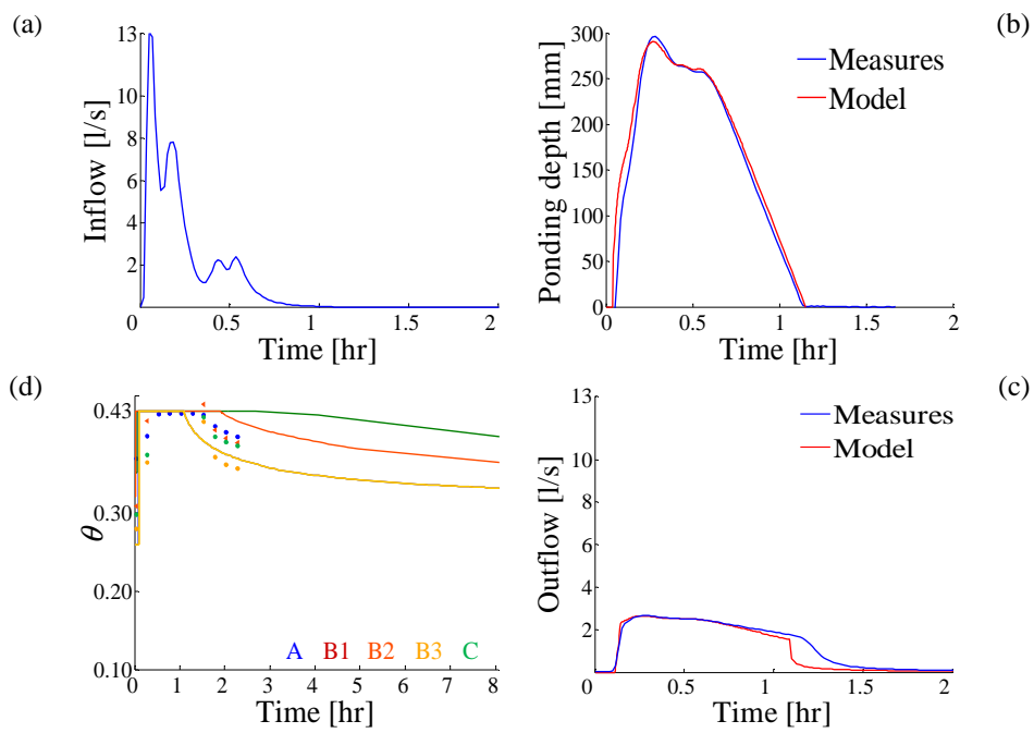
Fig. 75 – Event T*: (a) Inflow hydrograph, measures; (b) Pondering depth time serie, measures and model; (c) Outflow hydrograph, measures and model; (d) Soil moisture time series, measures and model
