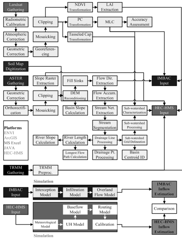
Figure 3: Methodology Flowchart.
