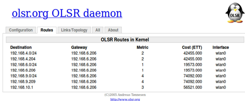
Figure 2: The (linear) topology of the network consisting of nodes 192.168.6.206, *.204, *.9.209, and *.10.1, as seen by the command centre. The drone (with IP address 192.168.10.1) is 3 hops away from the command centre and functions as a router. The ETT values indicate the cost of the links based on delay and loss.
