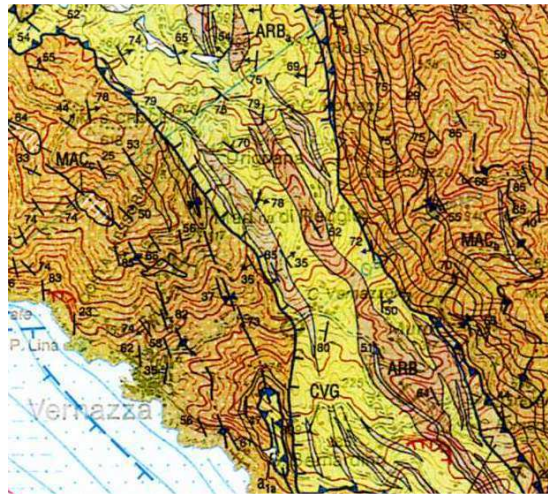
Figure 2: Geological map, Italy, Project CARG, Foglio 248, LaSpezia (2003).
