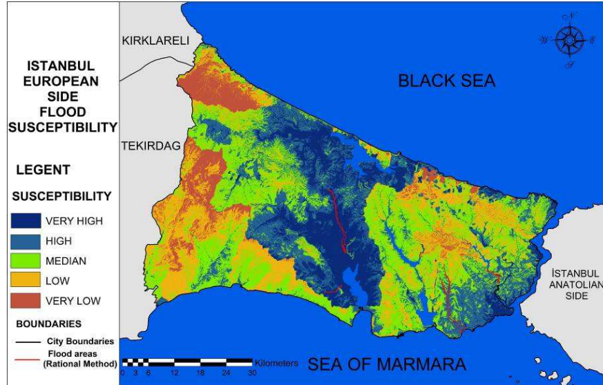
Figure 4: Classification maps.
