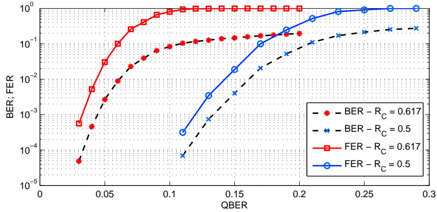
Figure 7.7: BER and FER performance of the LDPC decoders considered in Figures 7.3 and 7.5 as a function of Q for \alpha_Q = 1
