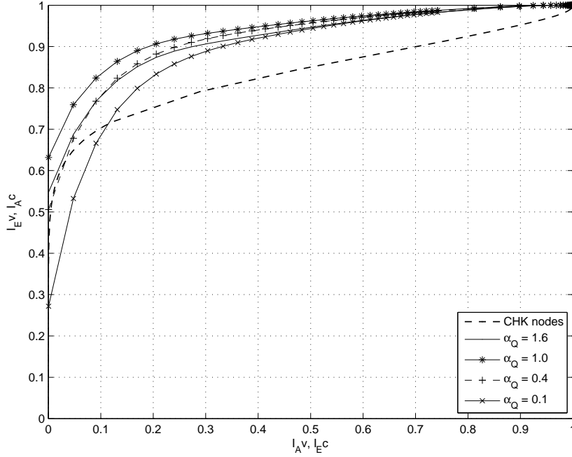
Figure 7.9: EXIT chart of the LDPC decoder considered (lower curve) as a function of \alpha_Q and for Q = 0.08
