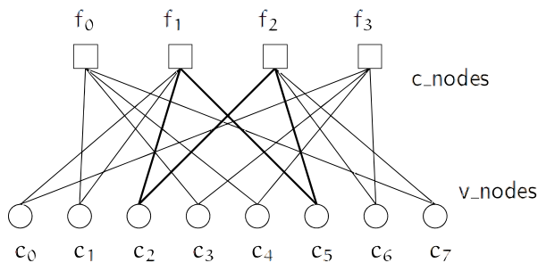
Figure 4.3: Tanner graph corresponding to the parity check matrix \mathbf{H} . The marked path c_2 \rightarrow f_1 \rightarrow c_5 \rightarrow f_2 \rightarrow c_2 is an example for a short cycle. Those should usually be avoided since they are bad for decoding performance.
