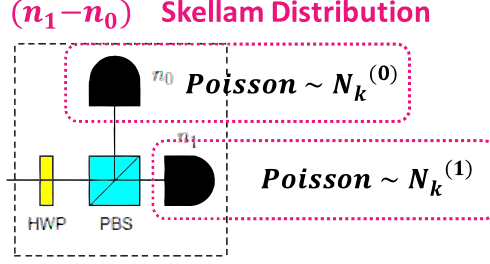
Figure 6.8: Decoding stage: Skellam distribution (n_1 - n_0)
