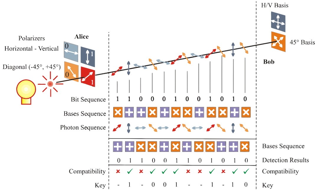
Figure 3.3: BB84 Protocol
