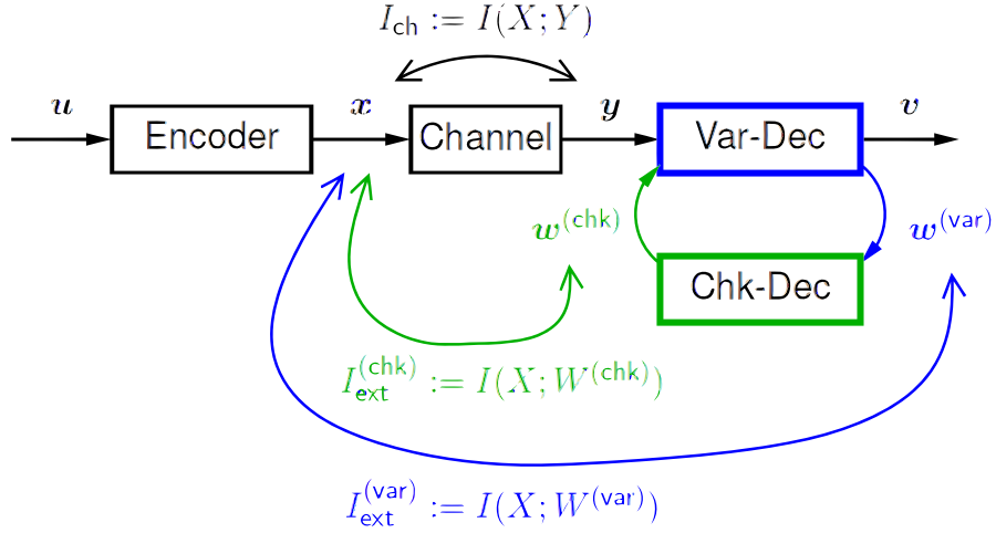
Figure 4.5: Block Diagram for the construction of LDPC EXIT Charts
