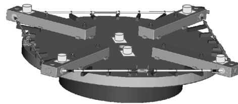
Figure 7. Schematic view of the G ring-laser. The device is mounted on a single block of zerodur, an extremely rigid and thermally stable ceramic material
