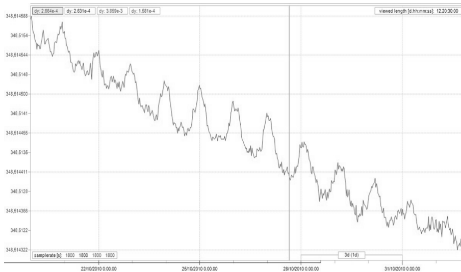
Figure 8. Signal from the G ring-laser during 13 days. Superposed to the Sagnac signal it can easily be seen the diurnal polar motion of the rotation axis of the Earth; the height of individual peaks is a bit less than 50 \mu Hz .
