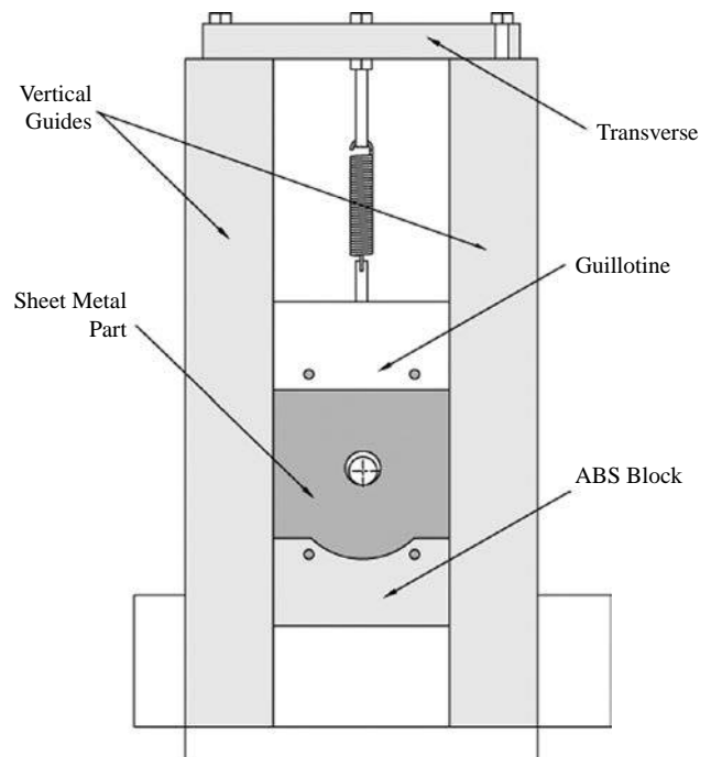
Figure 4 Detail of the reverse-guillotine
