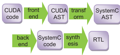
Figure 7. CUDA to FPGA flow
