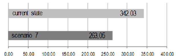
Fig. 13. Reductions of cooling loads due to roofs' insulation (MWh/year).
