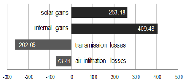
Fig. 6. Resumed variables involved on building's heat balance, which result in the building cooling load (MWh/year).
