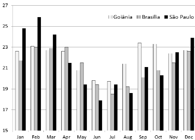
Fig. 3. Average monthly temperatures in Goiânia, Brasília and Sao Paulo.
