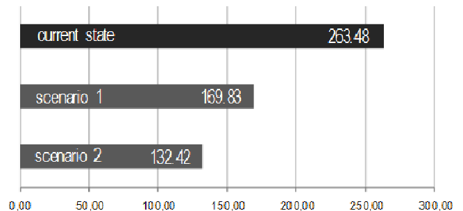
Fig. 7. Solar gains using different shading devices (MWh/year).
