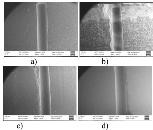
Figure 3: Cross-sections of the ZTA a) green and b) presintered, and c) green and d) presintered of AZT holes of the condition n°4.
