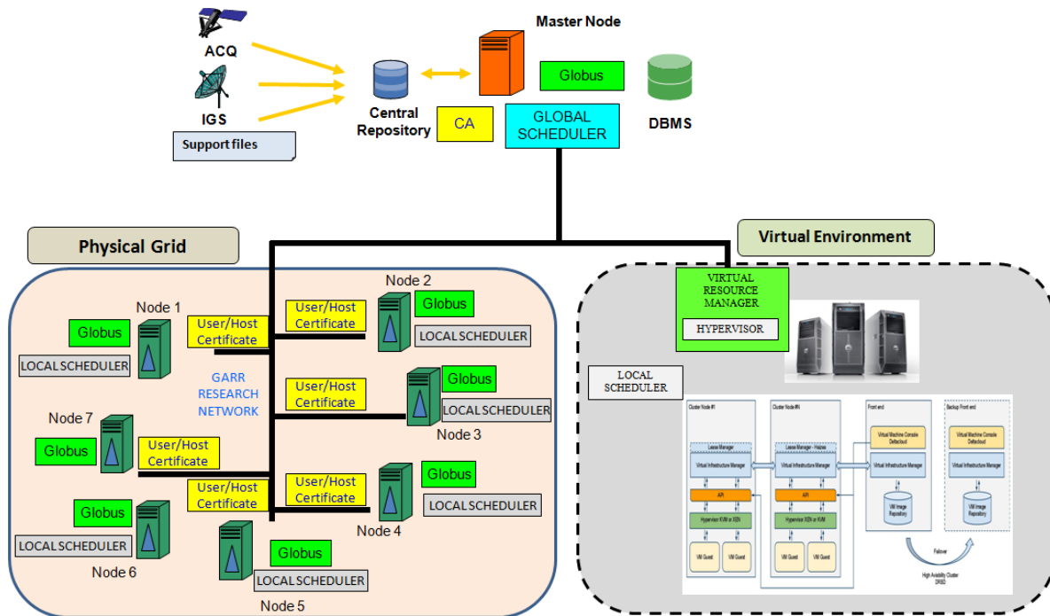
Figure 3. System Architecture.
