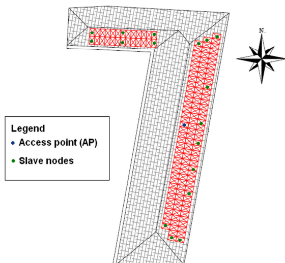
Figure 4. Plant of the first experimental WSN installed
