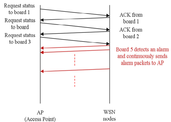
Figure 3. Example of a protocol transaction when a board detects an alarm
