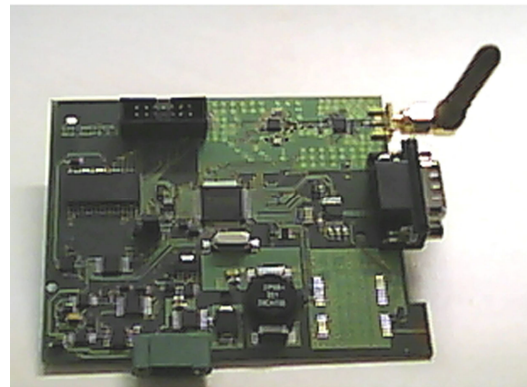
Figure 1. Sensor board used in the WSN
