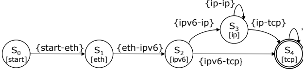
Fig. 9. Final DFA implementing the NetPFL filter of our example.
