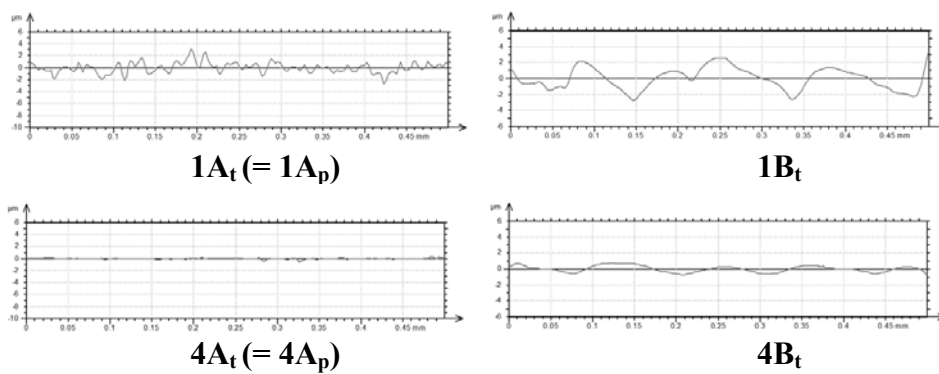
Fig. 6.7 2D PS profiles of sample 1 (up) and 4 (down), before (left) and after (right) thermoforming treatment. Each profile was extracted at 50 mm from the edge of the square measured area shown in Fig. 6.6.
