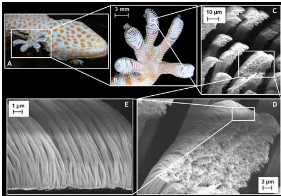
Fig. 1.1 The gecko's hierarchical adhesive apparatus. (A) Ventral view of the Tokay gecko ( Gekko gecko ). (B) Gecko's foot. Scanning electron microscope (SEM) micrographs of (C) the setae, (D) at higher magnification, (E) terminating in hundreds of spatula.
