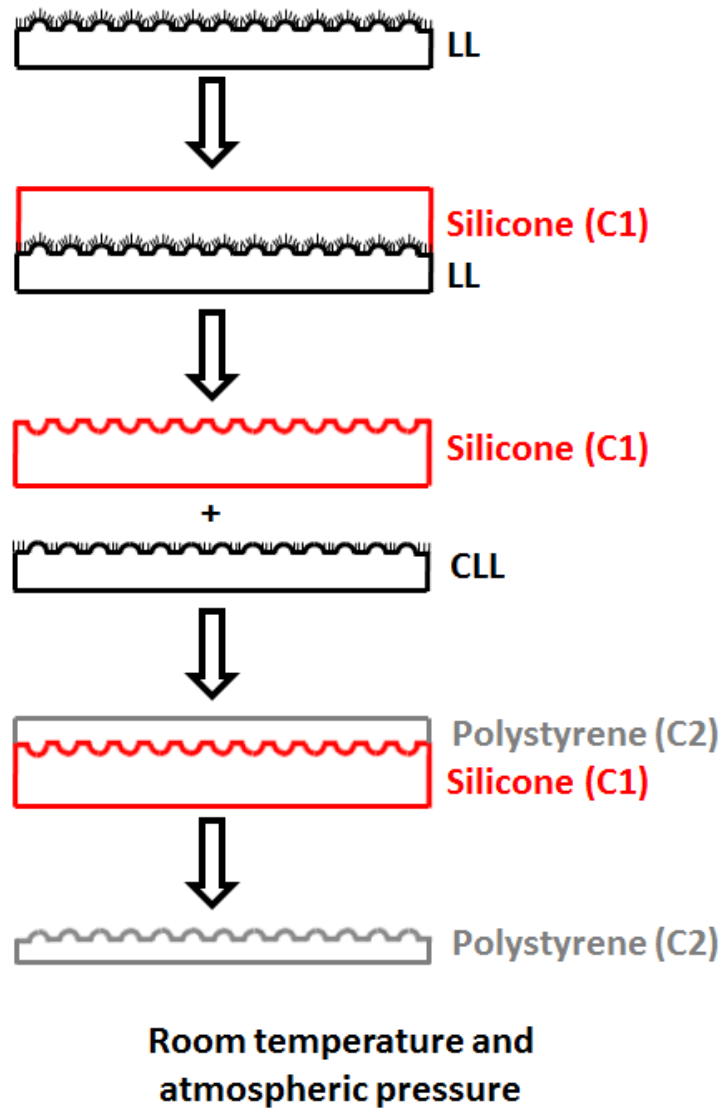
Fig. 7.1 Schematic illustration of our lotus leaf replication process, composed of two steps at room temperature and atmospheric pressure.
