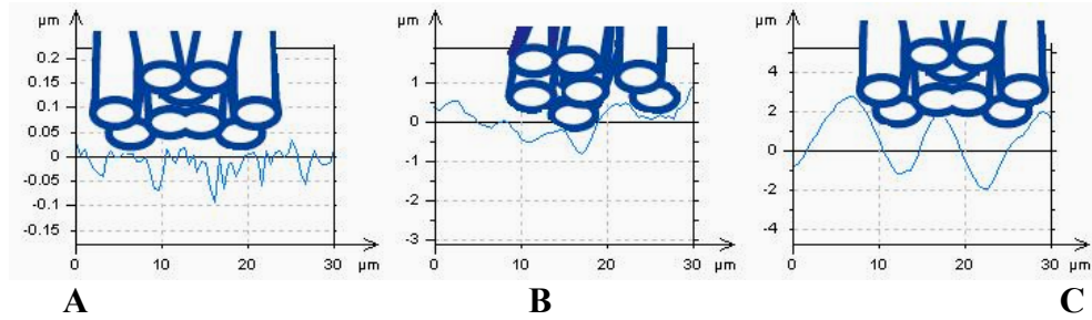
Fig. 1.10 Interpretation of experimental results of adhesion tests on different-roughness PMMA surfaces. (A) Setae (represented in blue) and its sub-hierarchical structures (spatulae) can adapt well on virgin PMMA; (B) on PMMA2400 surface the adhesion is better because of the higher interactions spatulae-substrates; (C) on PMMA800 only partial contact interactions are achieved.
