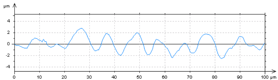
Fig. 1.6 PMMA800 surface. (A) Three-dimensional topography. (B) Two-dimensional profile (extracted at 50 \mu\text{m} from the edge of the square measured area).
